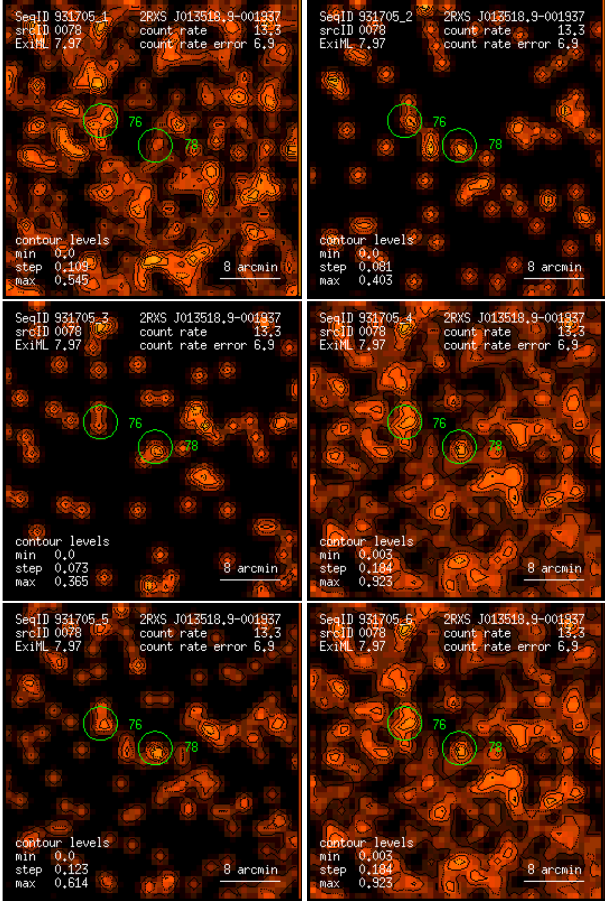
Figure 78: RASS 931705: detection 0078: band rate images, Gaussian filter: (1) PSPC channels 11 – 41, (2) 52 – 90, (3) 91 – 201, (4) 11 – 235, (5) 52 – 201, (6) 11 – 201. Broad band rates in counts/ks. Band rate contour levels in counts/ks/arcmin 2 .
