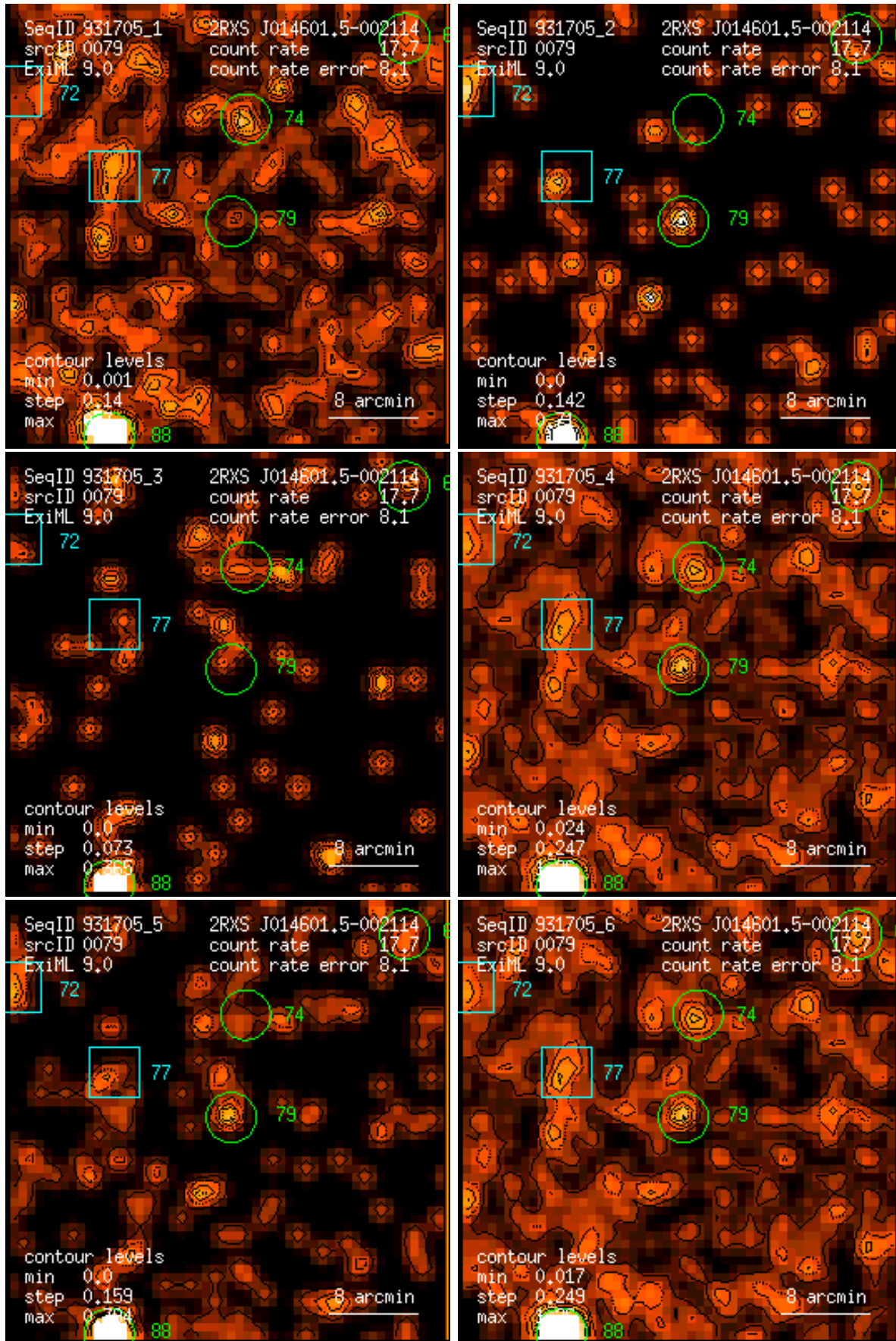
Figure 79: RASS 931705: detection 0079: band rate images, Gaussian filter: (1) PSPC channels 11 – 41, (2) 52 – 90, (3) 91 – 201, (4) 11 – 235, (5) 52 – 201, (6) 11 – 201. Broad band rates in counts/ks. Band rate contour levels in counts/ks/arcmin 2 .
