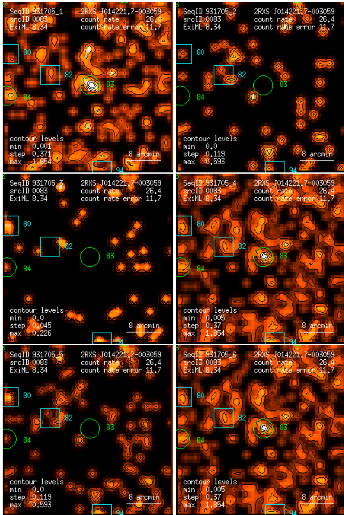
Figure 83: RASS 931705: detection 0083: band rate images, Gaussian filter: (1) PSPC channels 11 – 41, (2) 52 – 90, (3) 91 – 201, (4) 11 – 235, (5) 52 – 201, (6) 11 – 201. Broad band rates in counts/ks. Band rate contour levels in counts/ks/arcmin 2 .
