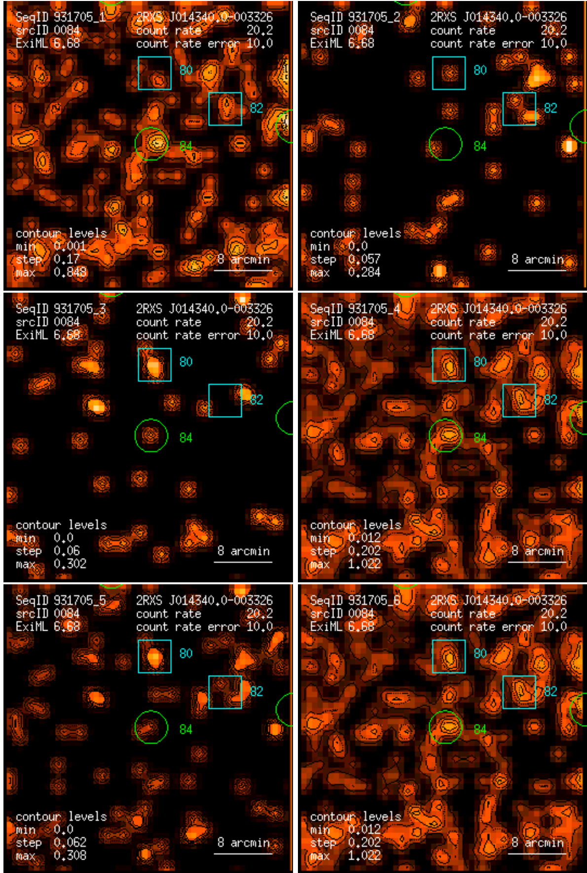
Figure 84: RASS 931705: detection 0084: band rate images, Gaussian filter: (1) PSPC channels 11 – 41, (2) 52 – 90, (3) 91 – 201, (4) 11 – 235, (5) 52 – 201, (6) 11 – 201. Broad band rates in counts/ks. Band rate contour levels in counts/ks/arcmin 2 .
