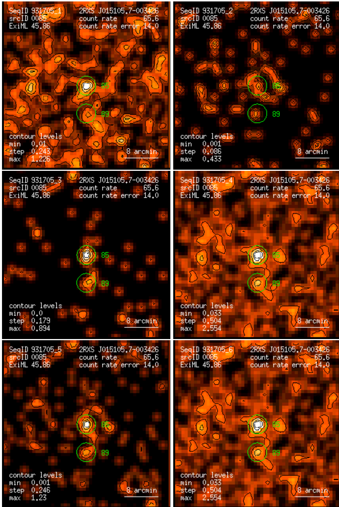
Figure 85: RASS 931705: detection 0085: band rate images, Gaussian filter: (1) PSPC channels 11 – 41, (2) 52 – 90, (3) 91 – 201, (4) 11 – 235, (5) 52 – 201, (6) 11 – 201. Broad band rates in counts/ks. Band rate contour levels in counts/ks/arcmin 2 .
