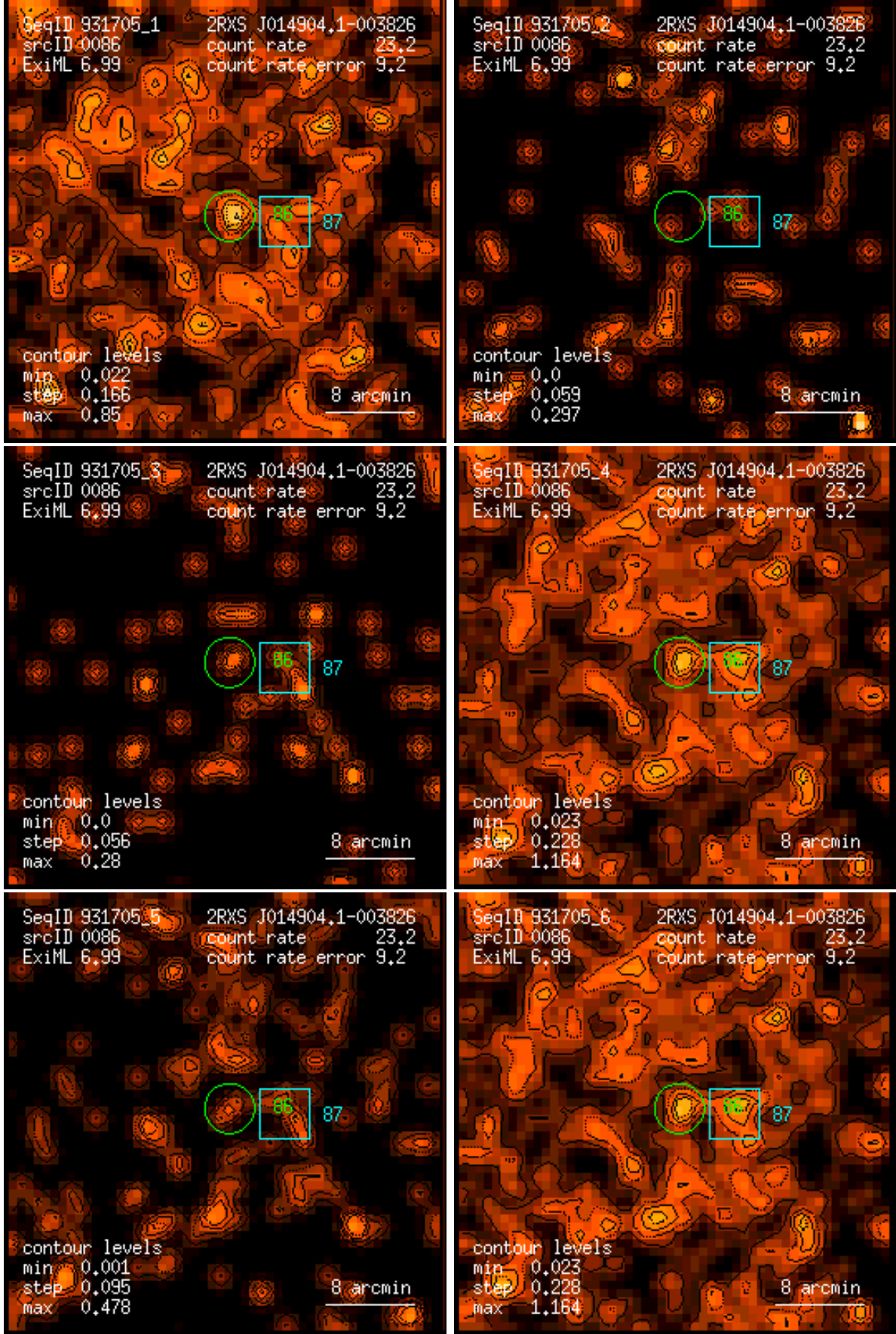
Figure 86: RASS 931705: detection 0086: band rate images, Gaussian filter: (1) PSPC channels 11 – 41, (2) 52 – 90, (3) 91 – 201, (4) 11 – 235, (5) 52 – 201, (6) 11 – 201. Broad band rates in counts/ks. Band rate contour levels in counts/ks/arcmin 2 .
