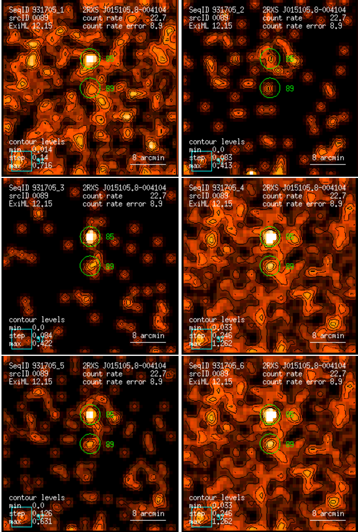
Figure 89: RASS 931705: detection 0089: band rate images, Gaussian filter: (1) PSPC channels 11 – 41, (2) 52 – 90, (3) 91 – 201, (4) 11 – 235, (5) 52 – 201, (6) 11 – 201. Broad band rates in counts/ks. Band rate contour levels in counts/ks/arcmin 2 .
