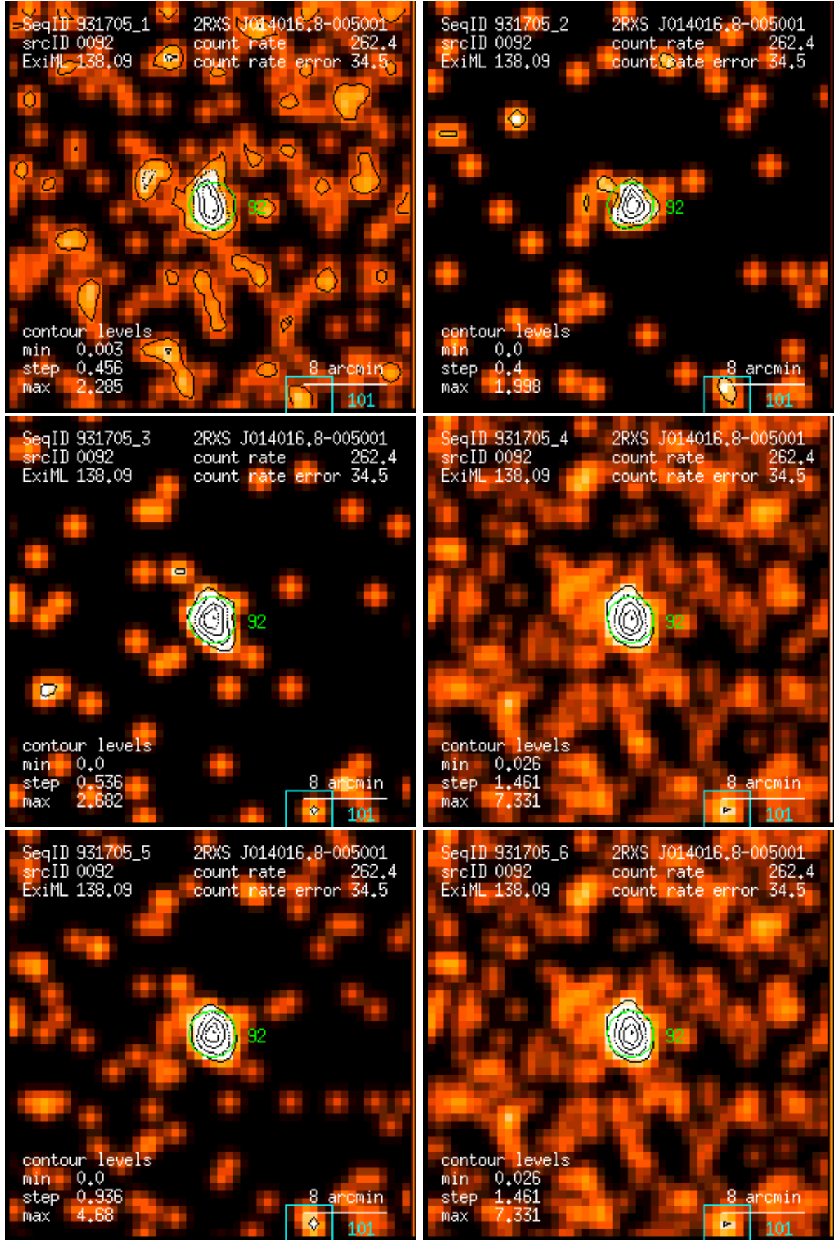
Figure 92: RASS 931705: detection 0092: band rate images, Gaussian filter: (1) PSPC channels 11 – 41, (2) 52 – 90, (3) 91 – 201, (4) 11 – 235, (5) 52 – 201, (6) 11 – 201. Broad band rates in counts/ks. Band rate contour levels in counts/ks/arcmin 2 .
