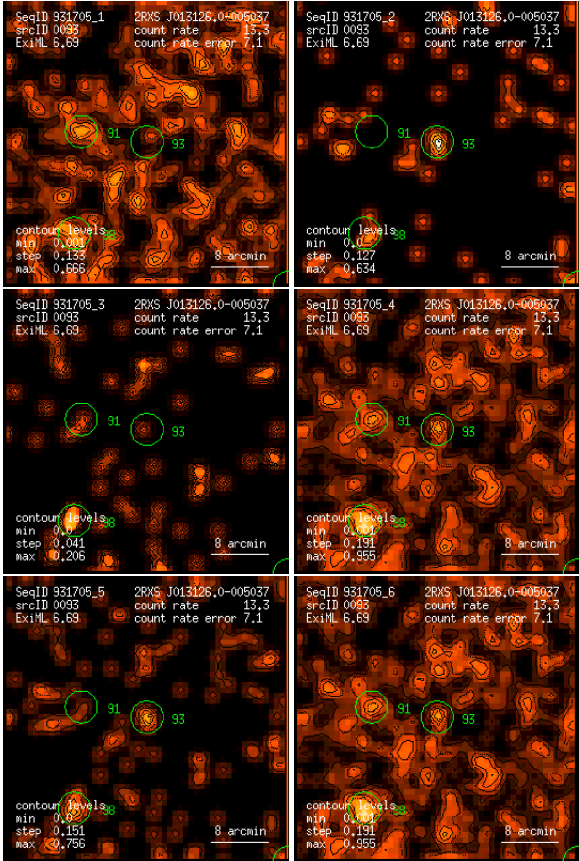
Figure 93: RASS 931705: detection 0093: band rate images, Gaussian filter: (1) PSPC channels 11 – 41, (2) 52 – 90, (3) 91 – 201, (4) 11 – 235, (5) 52 – 201, (6) 11 – 201. Broad band rates in counts/ks. Band rate contour levels in counts/ks/arcmin 2 .
