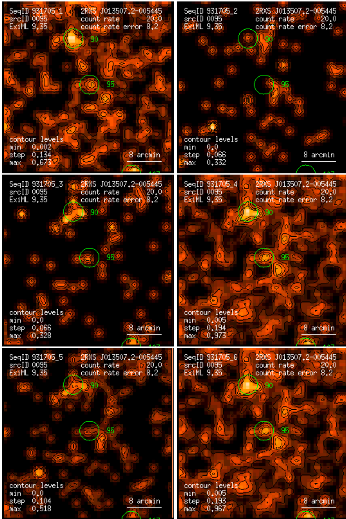
Figure 95: RASS 931705: detection 0095: band rate images, Gaussian filter: (1) PSPC channels 11 – 41, (2) 52 – 90, (3) 91 – 201, (4) 11 – 235, (5) 52 – 201, (6) 11 – 201. Broad band rates in counts/ks. Band rate contour levels in counts/ks/arcmin 2 .
