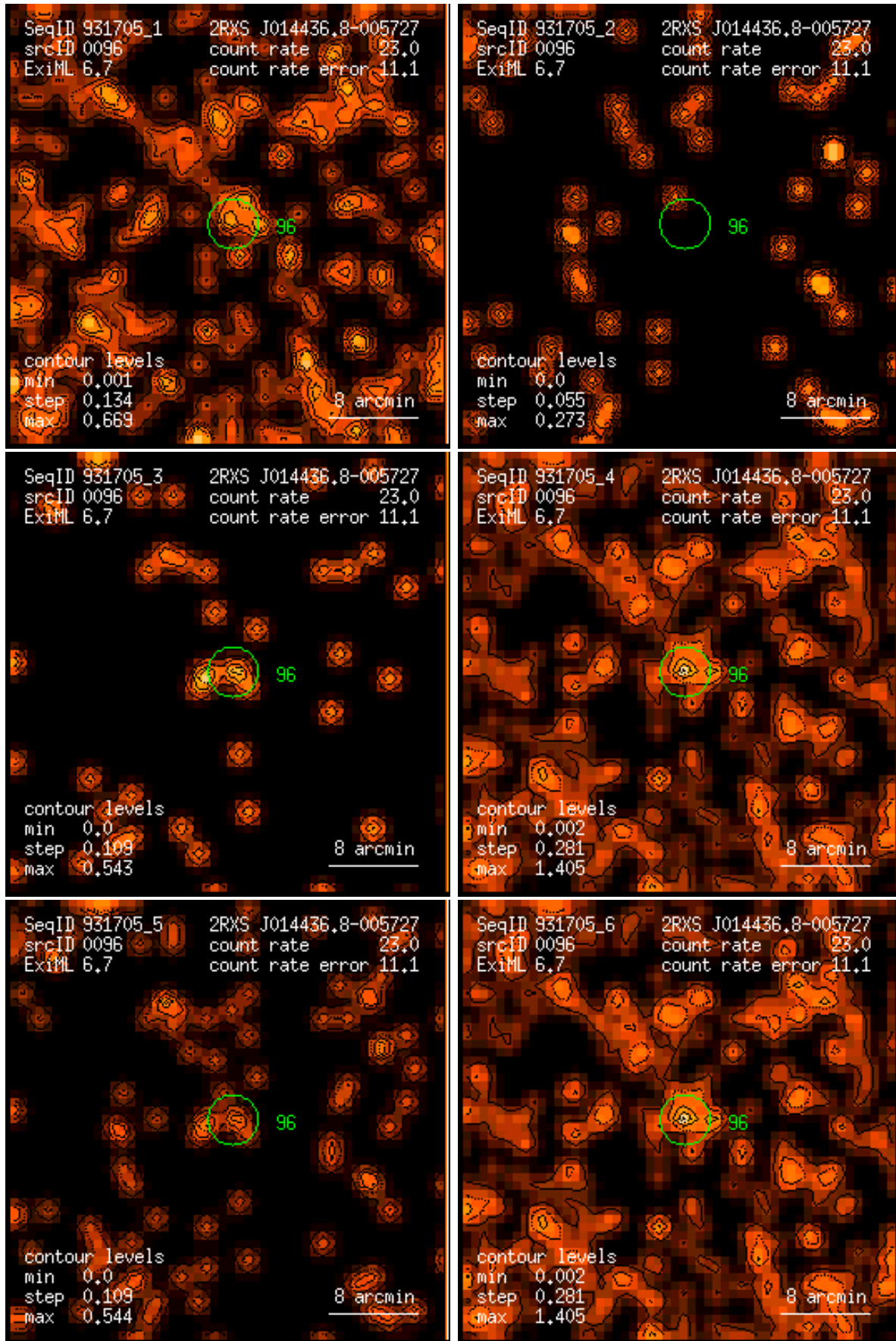
Figure 96: RASS 931705: detection 0096: band rate images, Gaussian filter: (1) PSPC channels 11 – 41, (2) 52 – 90, (3) 91 – 201, (4) 11 – 235, (5) 52 – 201, (6) 11 – 201. Broad band rates in counts/ks. Band rate contour levels in counts/ks/arcmin 2 .
