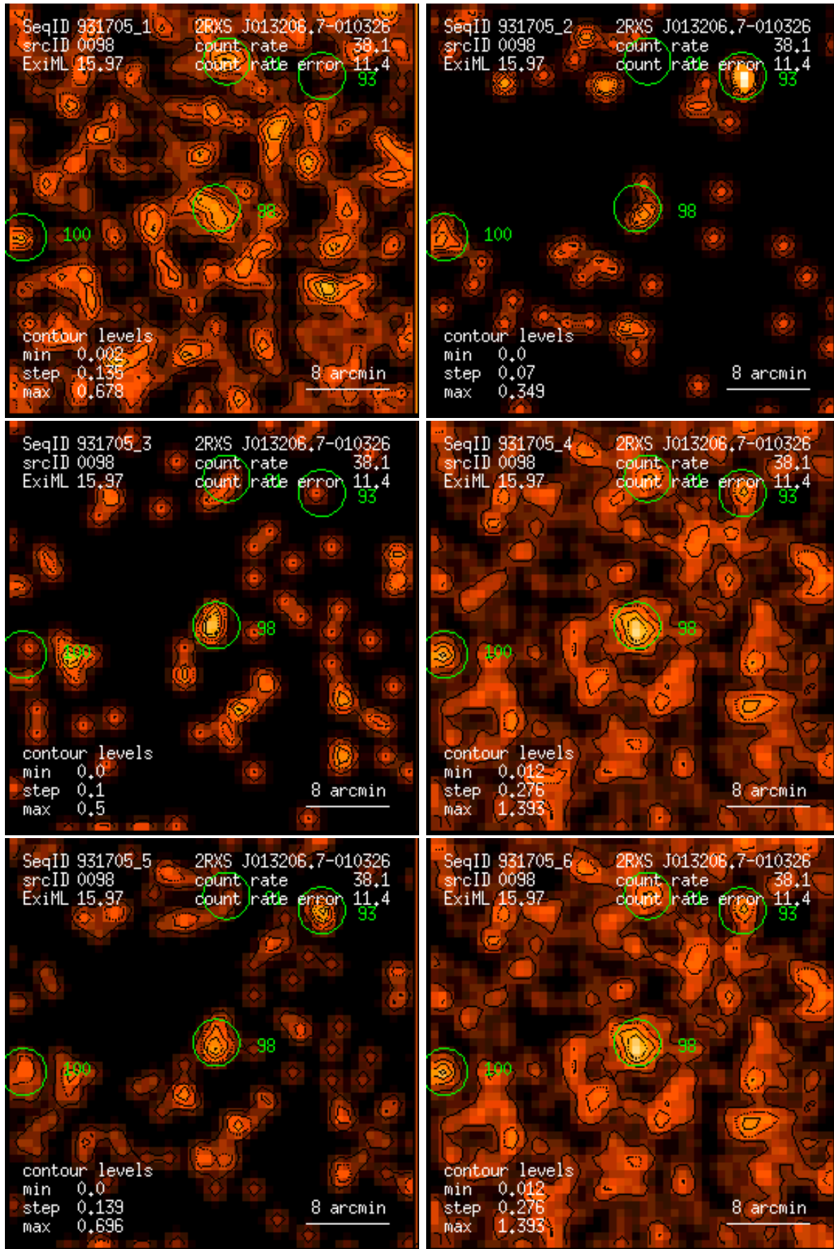
Figure 98: RASS 931705: detection 0098: band rate images, Gaussian filter: (1) PSPC channels 11 – 41, (2) 52 – 90, (3) 91 – 201, (4) 11 – 235, (5) 52 – 201, (6) 11 – 201. Broad band rates in counts/ks. Band rate contour levels in counts/ks/arcmin 2 .
