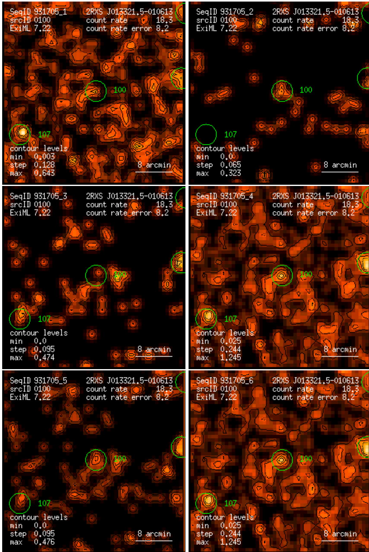
Figure 100: RASS 931705: detection 0100: band rate images, Gaussian filter: (1) PSPC channels 11 – 41, (2) 52 – 90, (3) 91 – 201, (4) 11 – 235, (5) 52 – 201, (6) 11 – 201. Broad band rates in counts/ks. Band rate contour levels in counts/ks/arcmin 2 .
