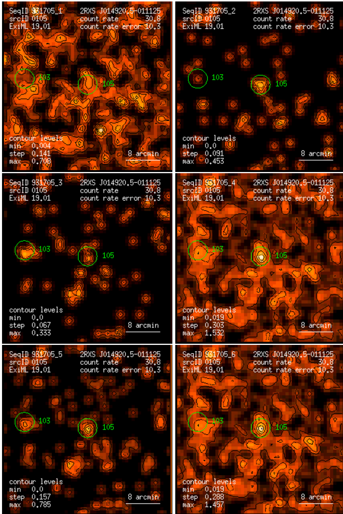
Figure 105: RASS 931705: detection 0105: band rate images, Gaussian filter: (1) PSPC channels 11 – 41, (2) 52 – 90, (3) 91 – 201, (4) 11 – 235, (5) 52 – 201, (6) 11 – 201. Broad band rates in counts/ks. Band rate contour levels in counts/ks/arcmin 2 .
