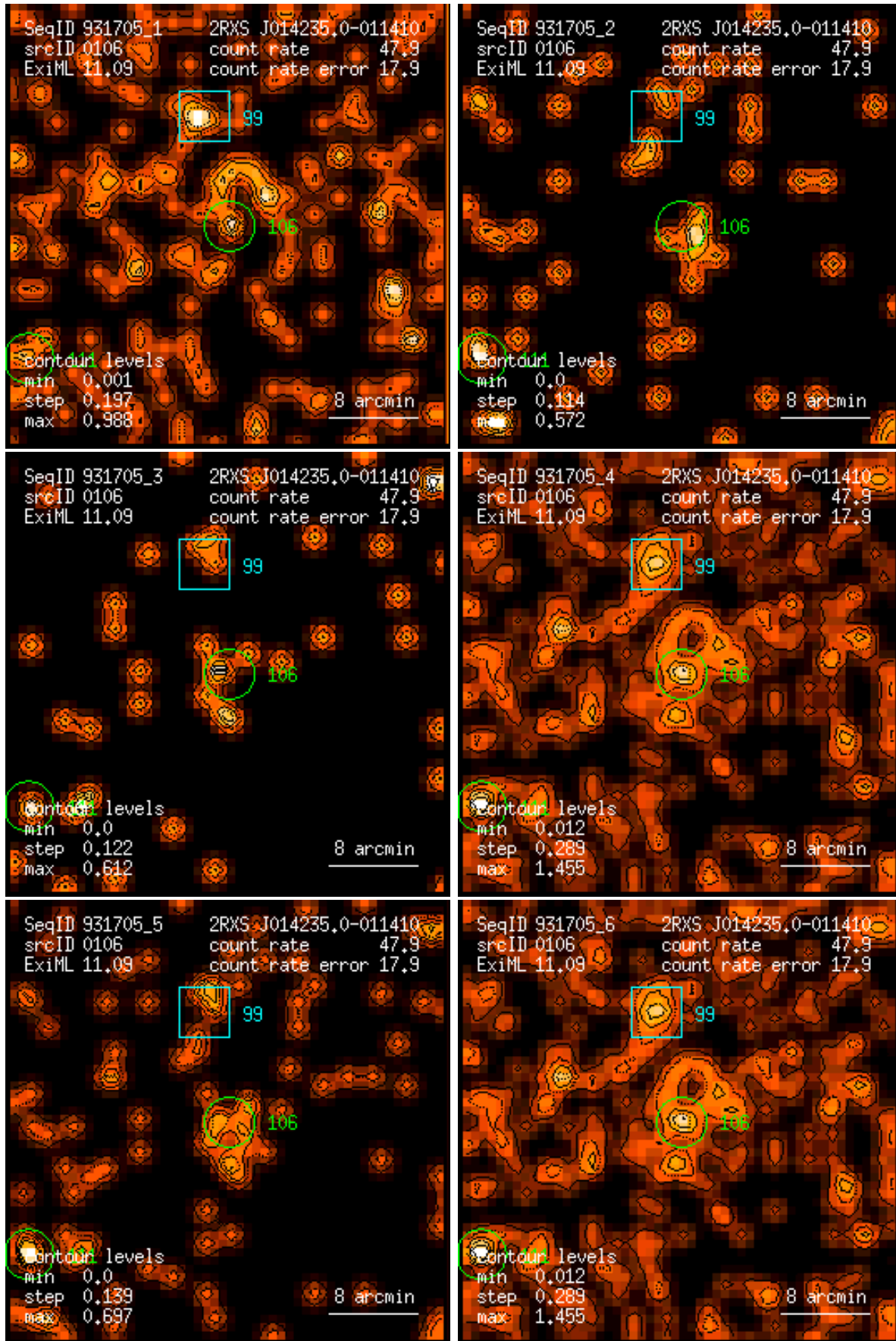
Figure 106: RASS 931705: detection 0106: band rate images, Gaussian filter: (1) PSPC channels 11 – 41, (2) 52 – 90, (3) 91 – 201, (4) 11 – 235, (5) 52 – 201, (6) 11 – 201. Broad band rates in counts/ks. Band rate contour levels in counts/ks/arcmin 2 .
