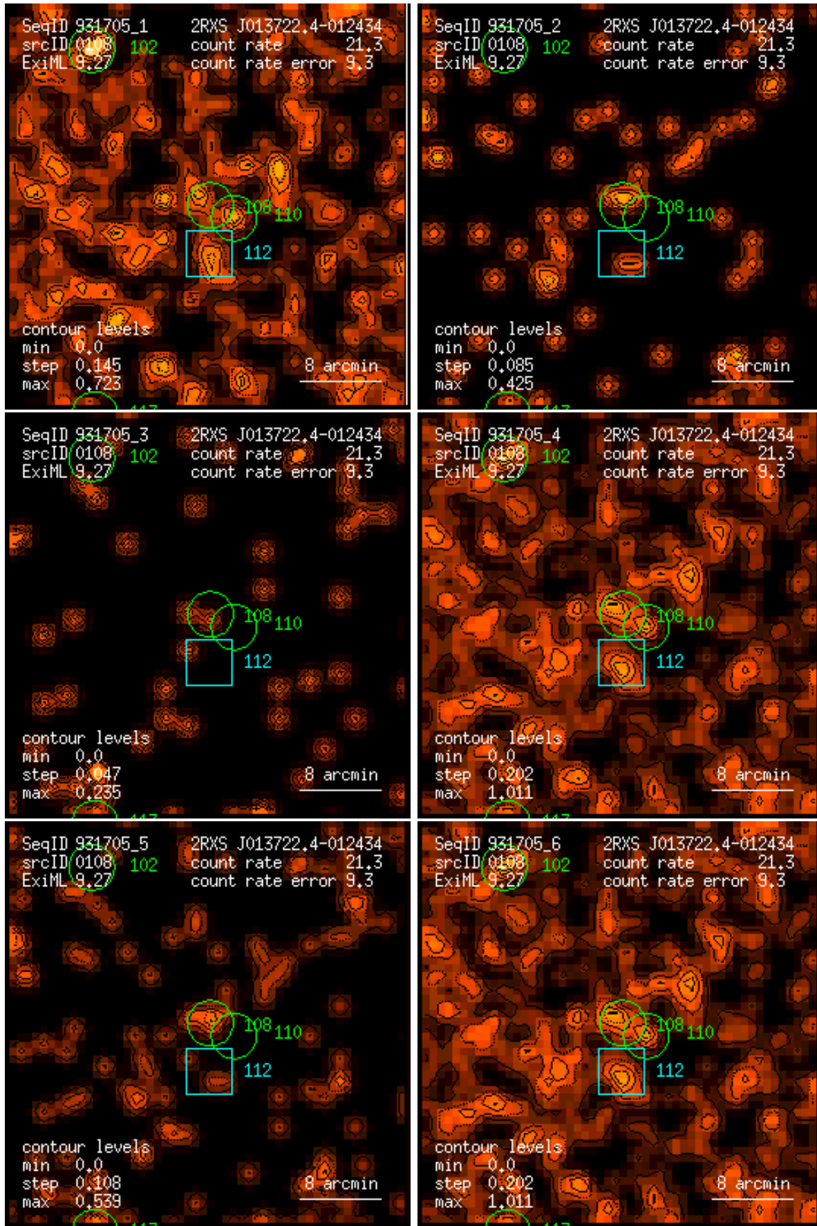
Figure 108: RASS 931705: detection 0108: band rate images, Gaussian filter: (1) PSPC channels 11 – 41, (2) 52 – 90, (3) 91 – 201, (4) 11 – 235, (5) 52 – 201, (6) 11 – 201. Broad band rates in counts/ks. Band rate contour levels in counts/ks/arcmin 2 .
