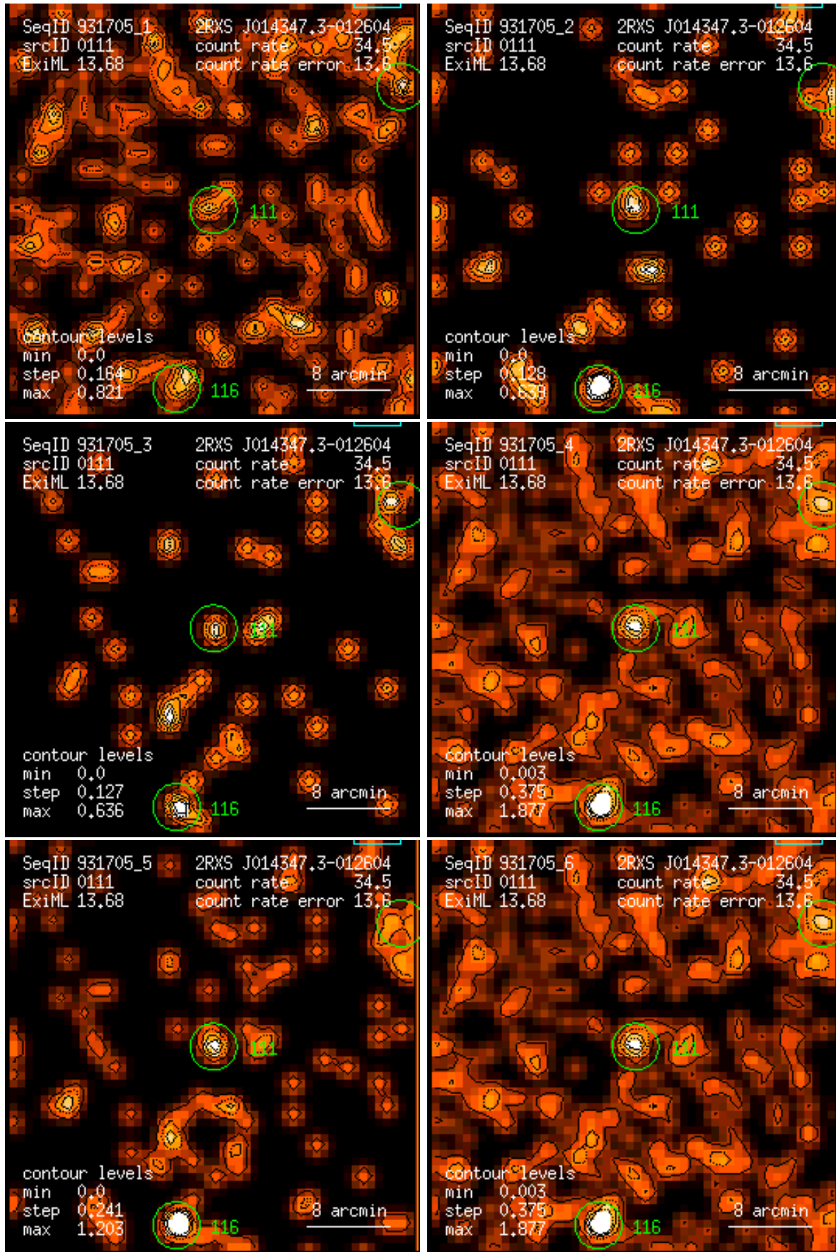
Figure 111: RASS 931705: detection 0111: band rate images, Gaussian filter: (1) PSPC channels 11 – 41, (2) 52 – 90, (3) 91 – 201, (4) 11 – 235, (5) 52 – 201, (6) 11 – 201. Broad band rates in counts/ks. Band rate contour levels in counts/ks/arcmin 2 .
