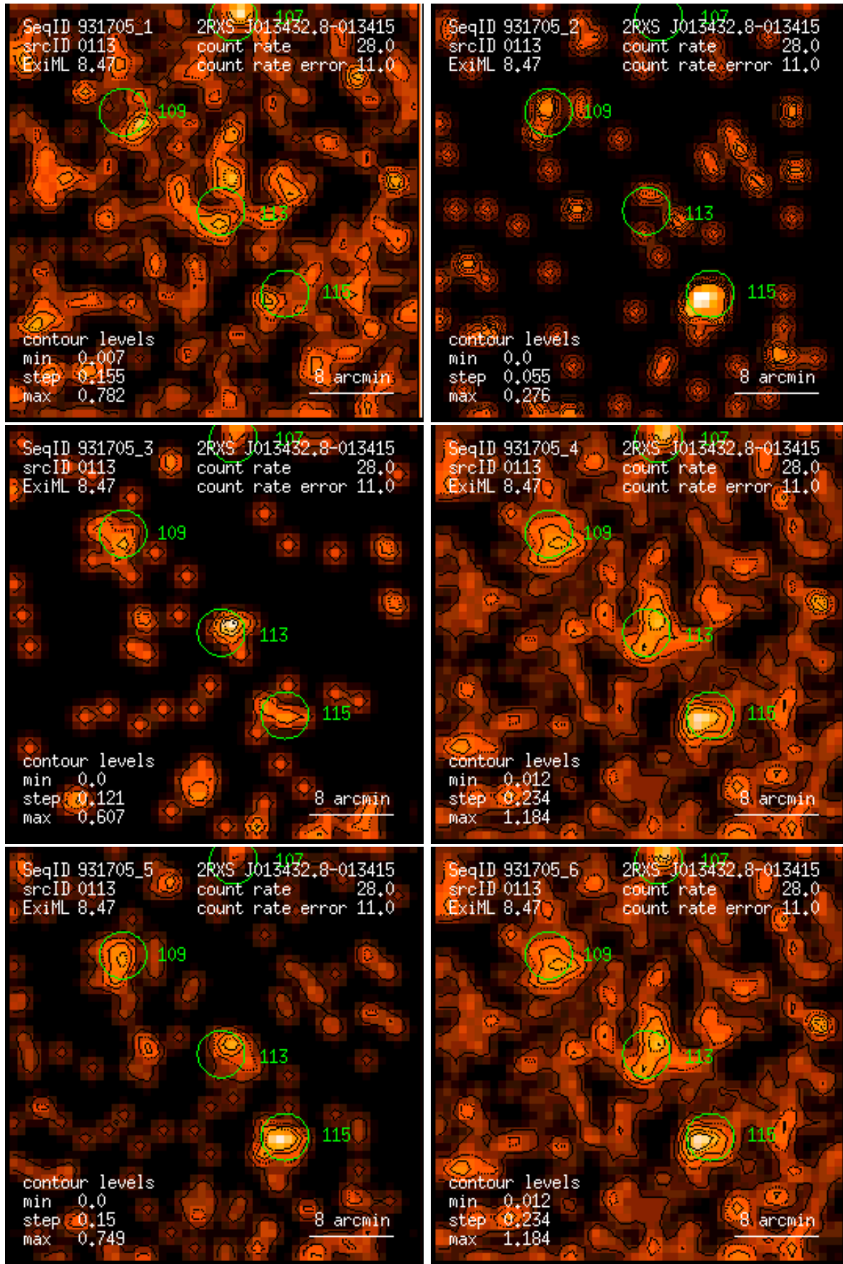
Figure 113: RASS 931705: detection 0113: band rate images, Gaussian filter: (1) PSPC channels 11 – 41, (2) 52 – 90, (3) 91 – 201, (4) 11 – 235, (5) 52 – 201, (6) 11 – 201. Broad band rates in counts/ks. Band rate contour levels in counts/ks/arcmin 2 .
