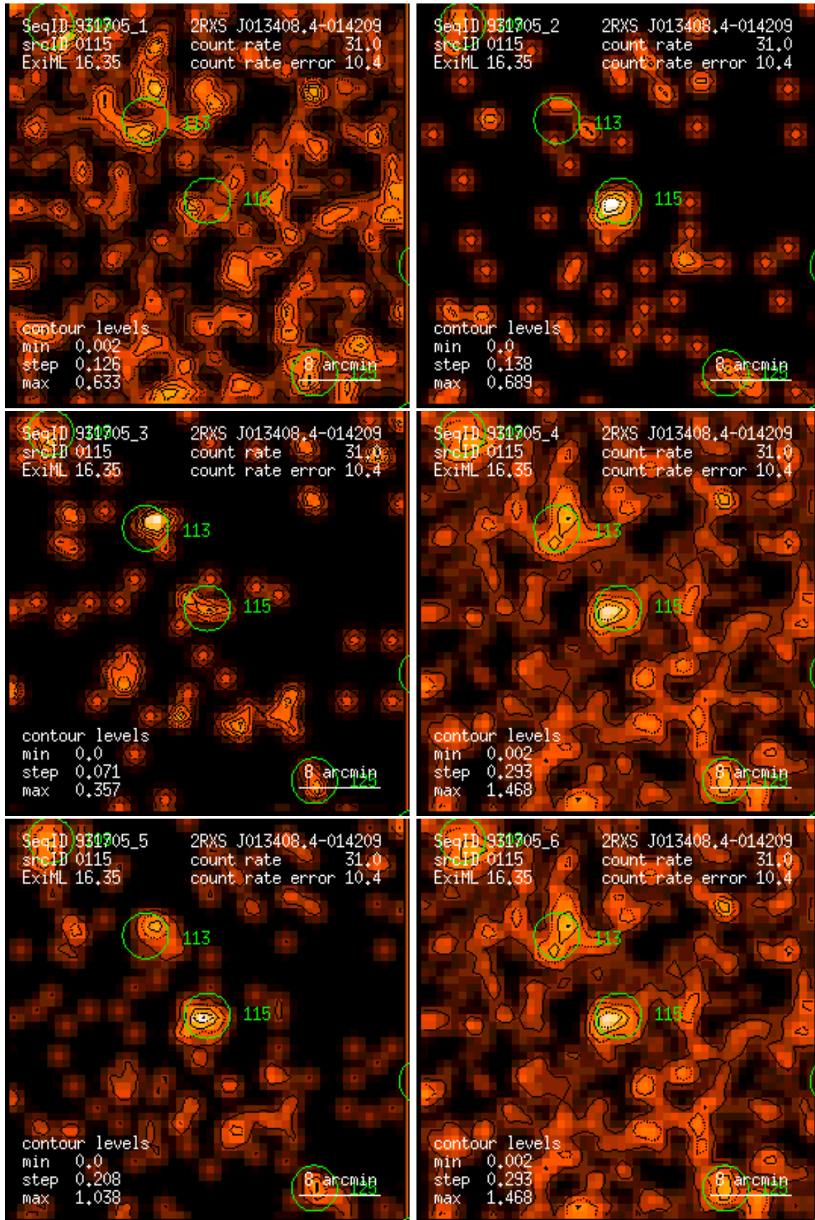
Figure 115: RASS 931705: detection 0115: band rate images, Gaussian filter: (1) PSPC channels 11 – 41, (2) 52 – 90, (3) 91 – 201, (4) 11 – 235, (5) 52 – 201, (6) 11 – 201. Broad band rates in counts/ks. Band rate contour levels in counts/ks/arcmin 2 .
