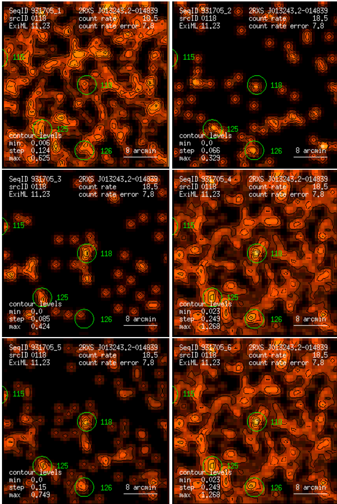
Figure 118: RASS 931705: detection 0118: band rate images, Gaussian filter: (1) PSPC channels 11 – 41, (2) 52 – 90, (3) 91 – 201, (4) 11 – 235, (5) 52 – 201, (6) 11 – 201. Broad band rates in counts/ks. Band rate contour levels in counts/ks/arcmin 2 .
