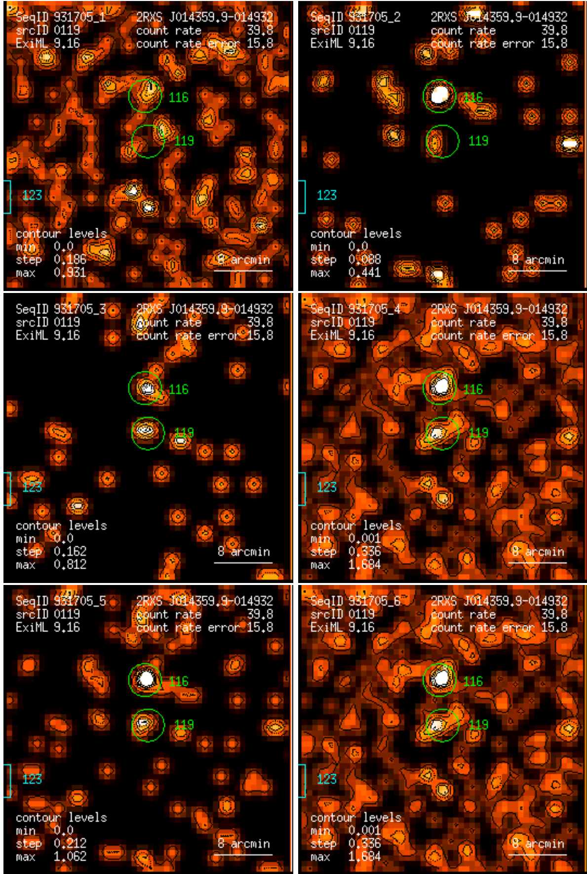
Figure 119: RASS 931705: detection 0119: band rate images, Gaussian filter: (1) PSPC channels 11 – 41, (2) 52 – 90, (3) 91 – 201, (4) 11 – 235, (5) 52 – 201, (6) 11 – 201. Broad band rates in counts/ks. Band rate contour levels in counts/ks/arcmin 2 .
