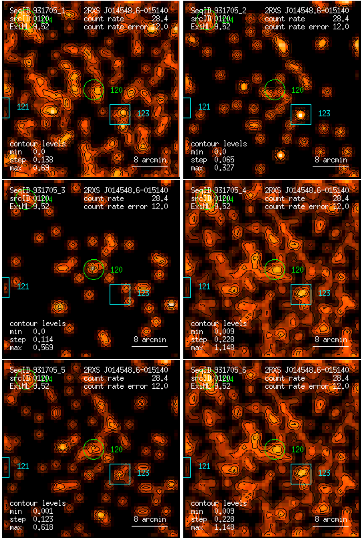
Figure 120: RASS 931705: detection 0120: band rate images, Gaussian filter: (1) PSPC channels 11 – 41, (2) 52 – 90, (3) 91 – 201, (4) 11 – 235, (5) 52 – 201, (6) 11 – 201. Broad band rates in counts/ks. Band rate contour levels in counts/ks/arcmin 2 .
