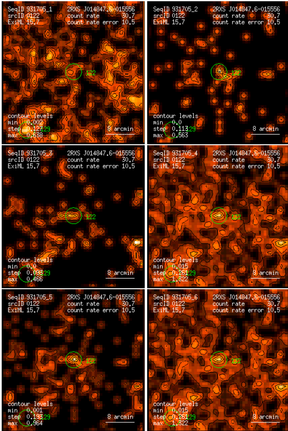
Figure 122: RASS 931705: detection 0122: band rate images, Gaussian filter: (1) PSPC channels 11 – 41, (2) 52 – 90, (3) 91 – 201, (4) 11 – 235, (5) 52 – 201, (6) 11 – 201. Broad band rates in counts/ks. Band rate contour levels in counts/ks/arcmin 2 .
