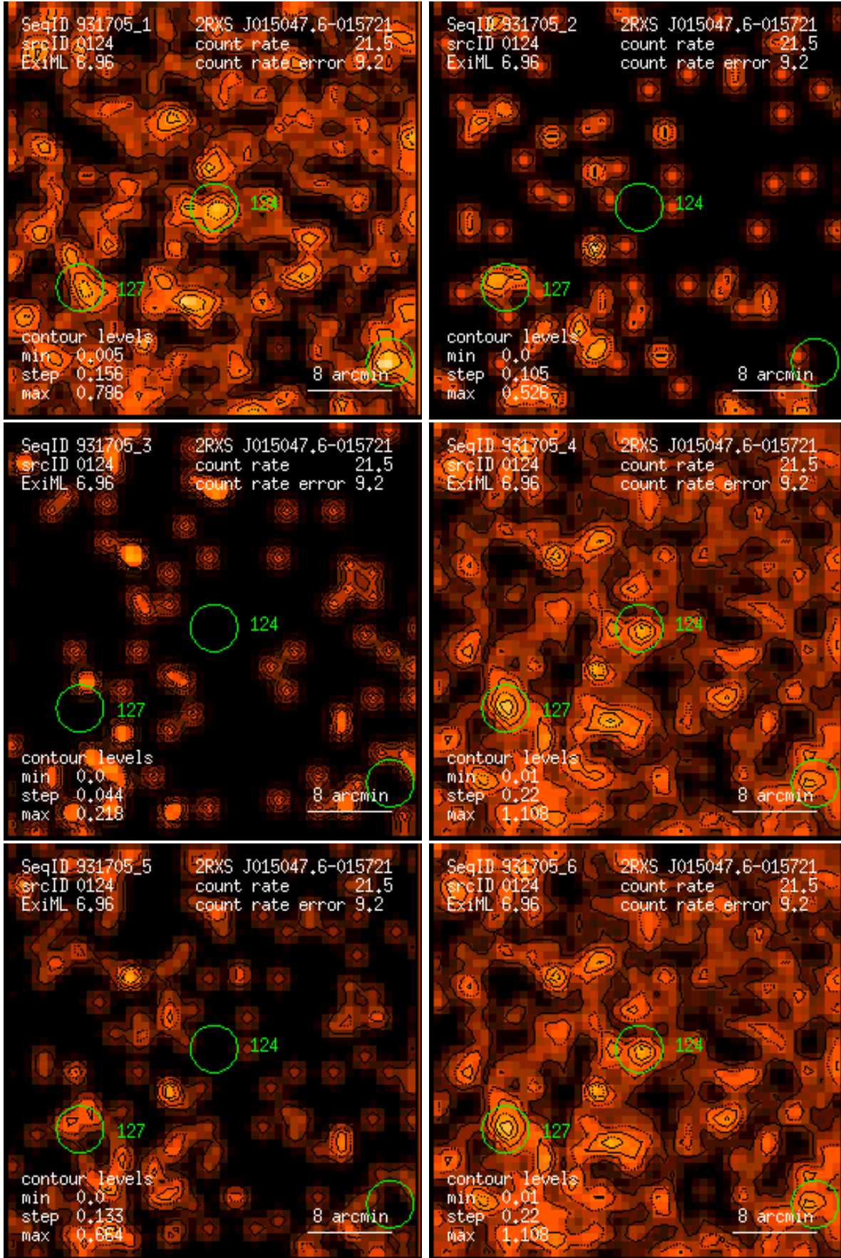
Figure 124: RASS 931705: detection 0124: band rate images, Gaussian filter: (1) PSPC channels 11 – 41, (2) 52 – 90, (3) 91 – 201, (4) 11 – 235, (5) 52 – 201, (6) 11 – 201. Broad band rates in counts/ks. Band rate contour levels in counts/ks/arcmin 2 .
