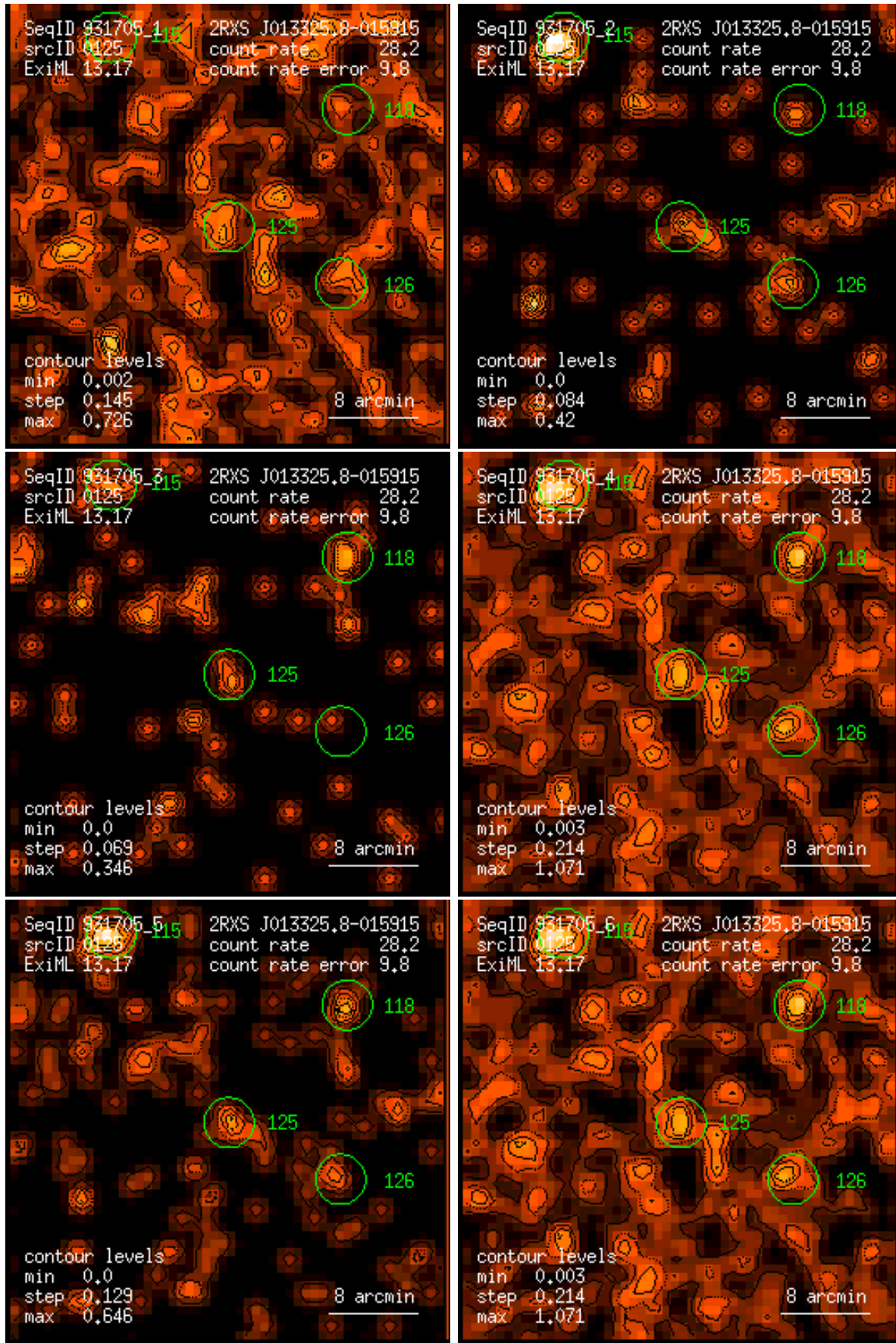
Figure 125: RASS 931705: detection 0125: band rate images, Gaussian filter: (1) PSPC channels 11 – 41, (2) 52 – 90, (3) 91 – 201, (4) 11 – 235, (5) 52 – 201, (6) 11 – 201. Broad band rates in counts/ks. Band rate contour levels in counts/ks/arcmin 2 .
