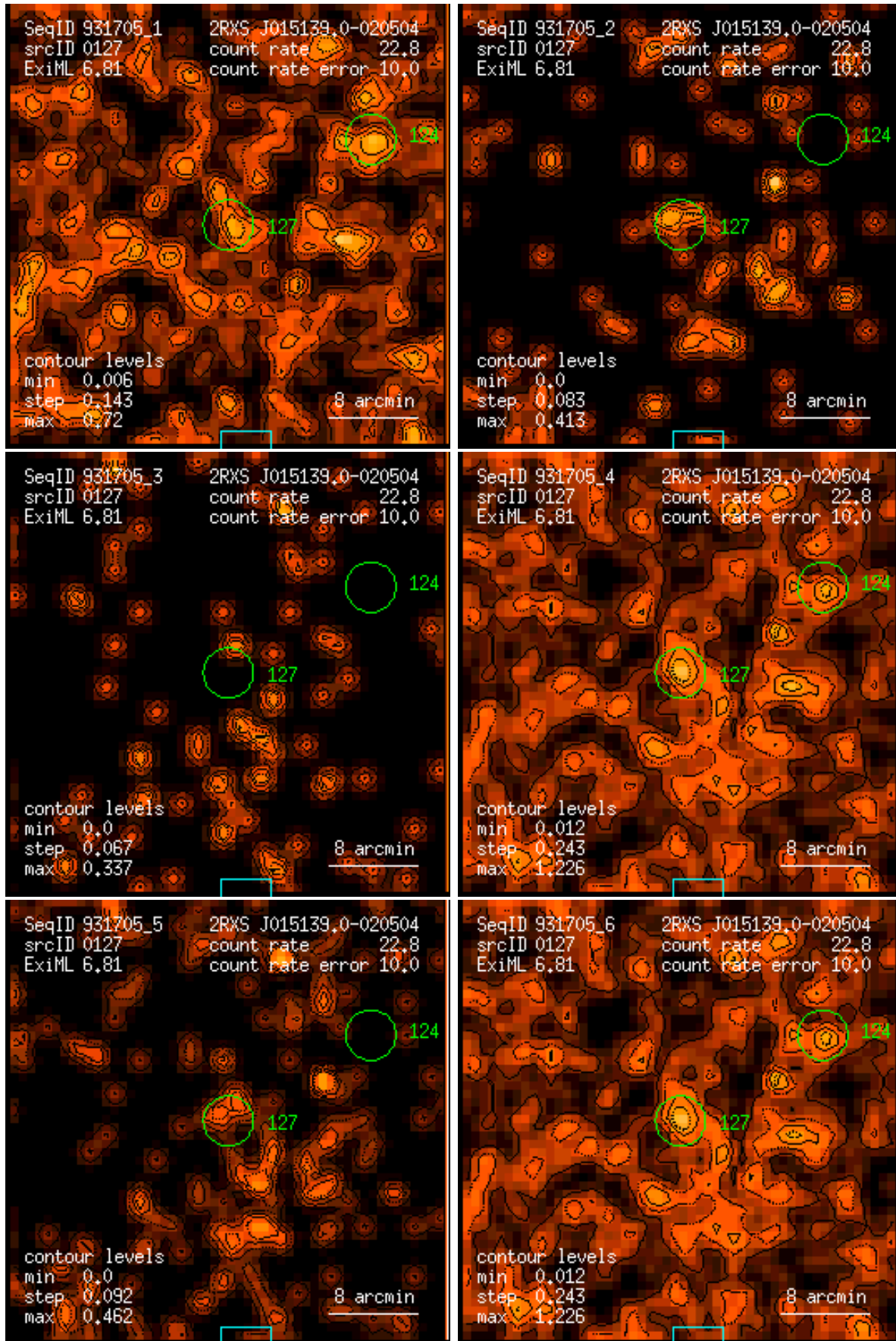
Figure 127: RASS 931705: detection 0127: band rate images, Gaussian filter: (1) PSPC channels 11 – 41, (2) 52 – 90, (3) 91 – 201, (4) 11 – 235, (5) 52 – 201, (6) 11 – 201. Broad band rates in counts/ks. Band rate contour levels in counts/ks/arcmin 2 .
