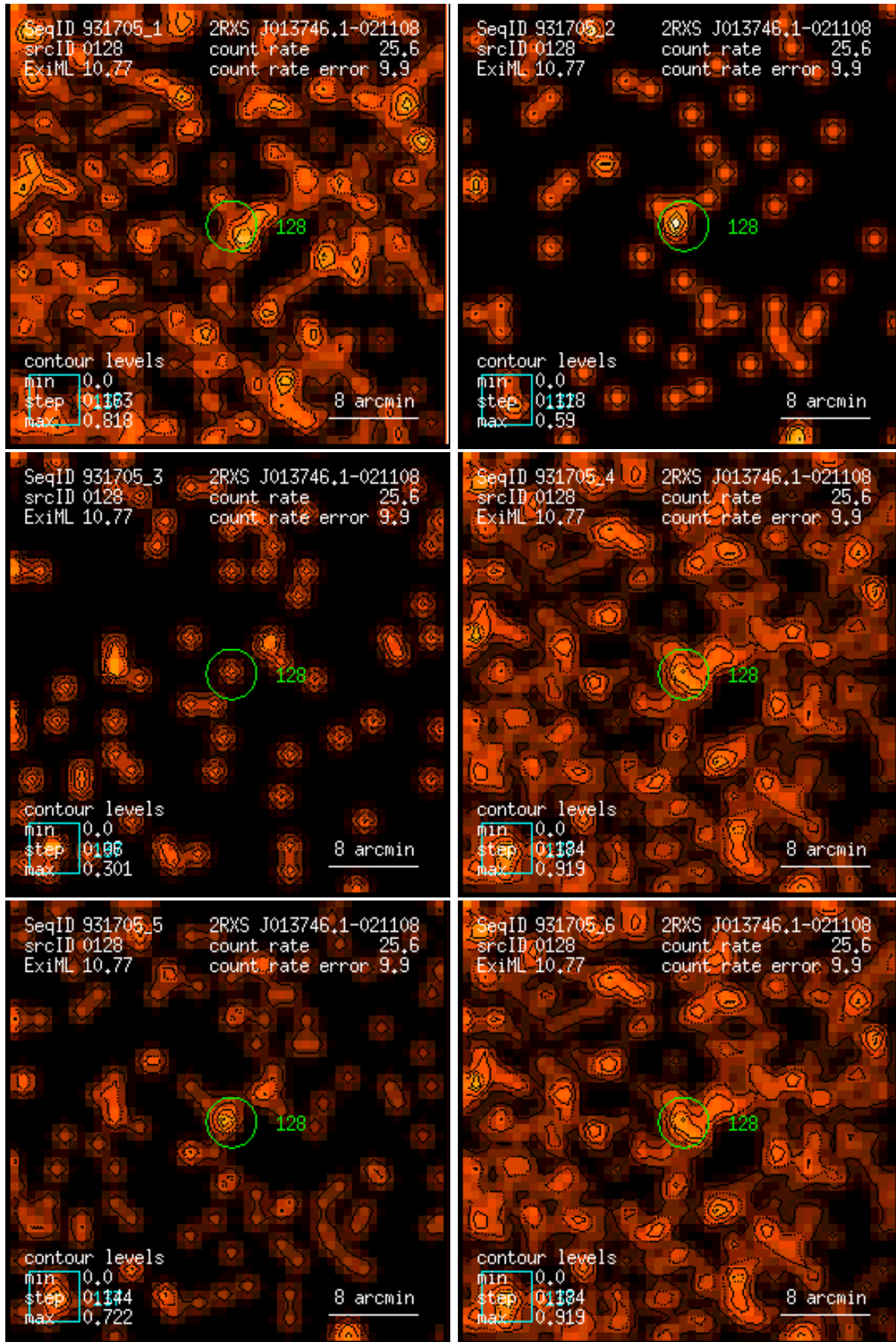
Figure 128: RASS 931705: detection 0128: band rate images, Gaussian filter: (1) PSPC channels 11 – 41, (2) 52 – 90, (3) 91 – 201, (4) 11 – 235, (5) 52 – 201, (6) 11 – 201. Broad band rates in counts/ks. Band rate contour levels in counts/ks/arcmin 2 .
