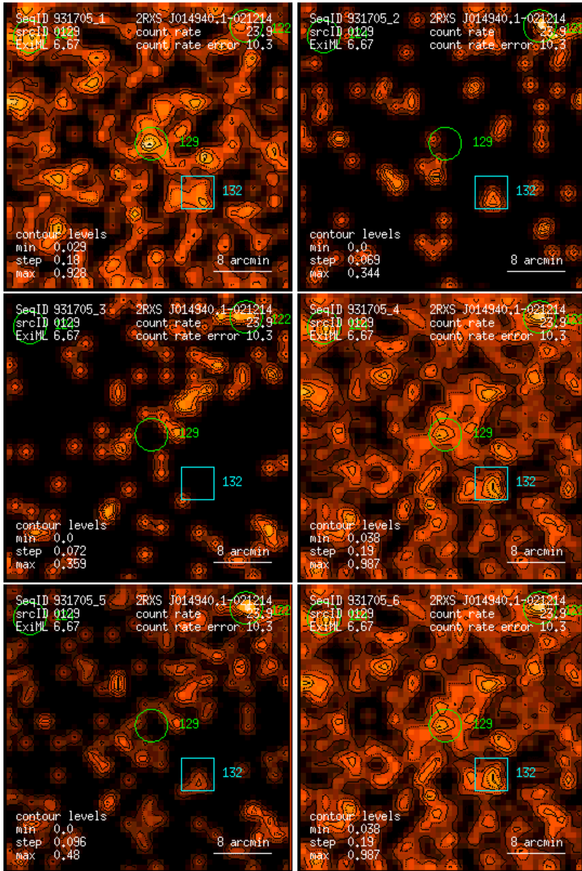
Figure 129: RASS 931705: detection 0129: band rate images, Gaussian filter: (1) PSPC channels 11 – 41, (2) 52 – 90, (3) 91 – 201, (4) 11 – 235, (5) 52 – 201, (6) 11 – 201. Broad band rates in counts/ks. Band rate contour levels in counts/ks/arcmin 2 .
