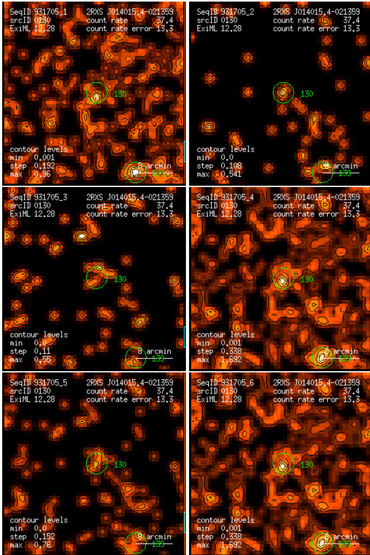
Figure 130: RASS 931705: detection 0130: band rate images, Gaussian filter: (1) PSPC channels 11 – 41, (2) 52 – 90, (3) 91 – 201, (4) 11 – 235, (5) 52 – 201, (6) 11 – 201. Broad band rates in counts/ks. Band rate contour levels in counts/ks/arcmin 2 .
