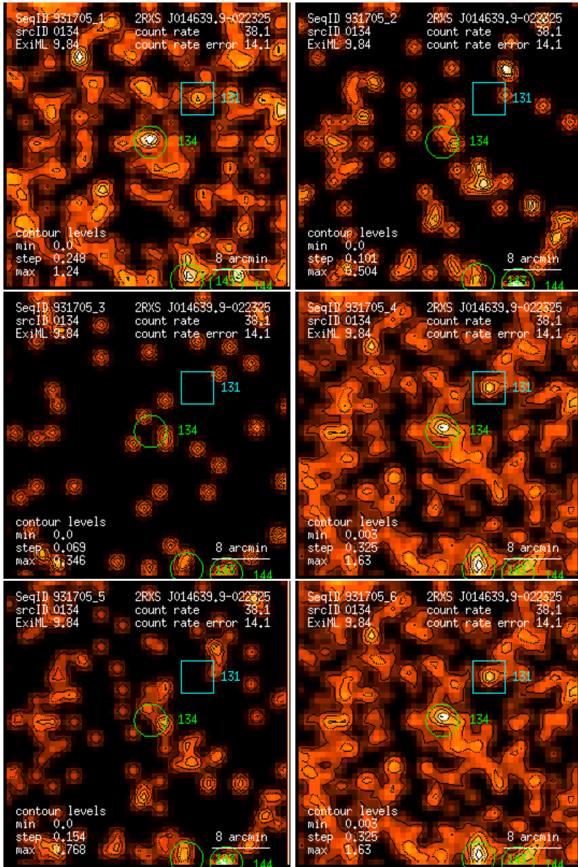
Figure 134: RASS 931705: detection 0134: band rate images, Gaussian filter: (1) PSPC channels 11 – 41, (2) 52 – 90, (3) 91 – 201, (4) 11 – 235, (5) 52 – 201, (6) 11 – 201. Broad band rates in counts/ks. Band rate contour levels in counts/ks/arcmin 2 .
