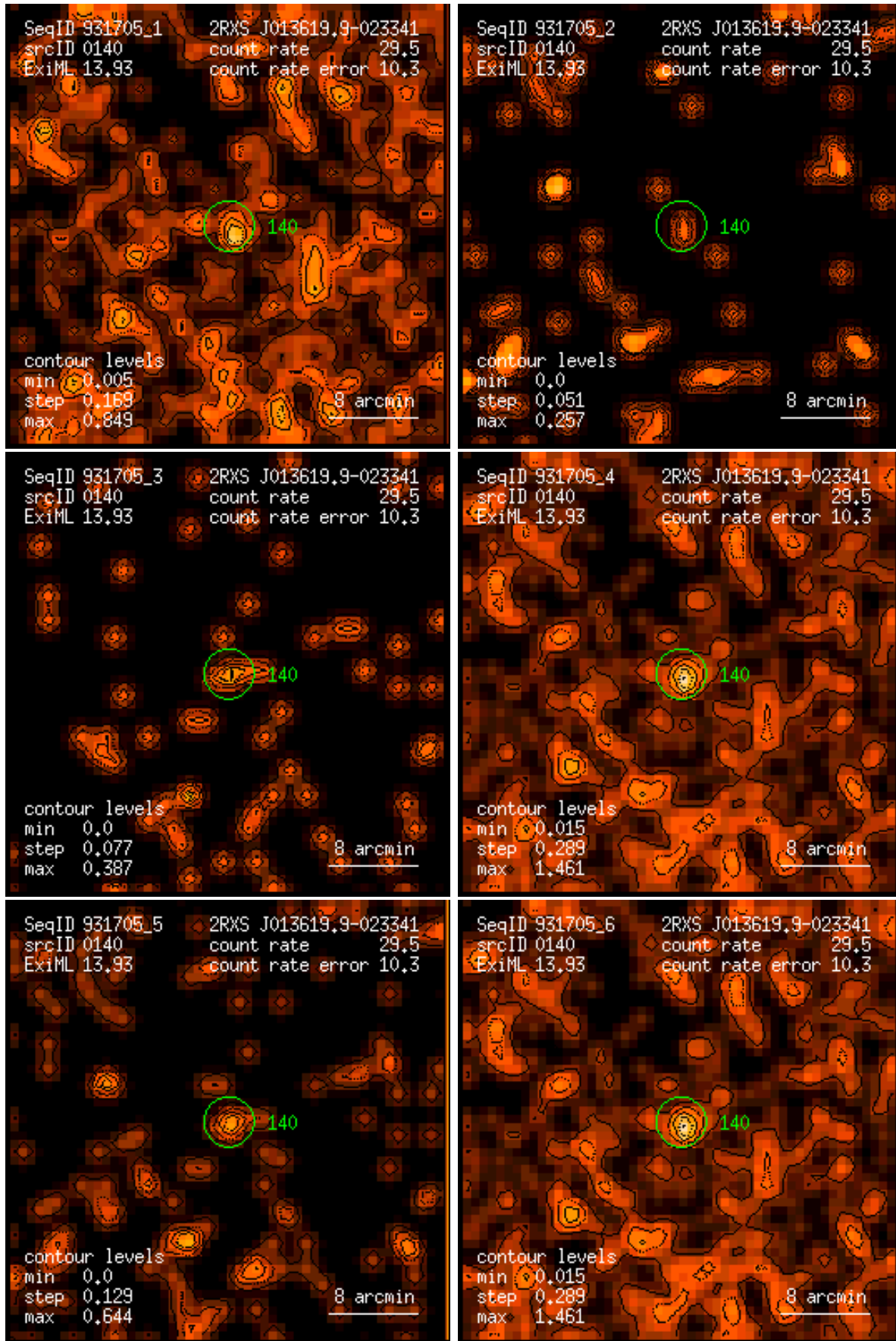
Figure 140: RASS 931705: detection 0140: band rate images, Gaussian filter: (1) PSPC channels 11 – 41, (2) 52 – 90, (3) 91 – 201, (4) 11 – 235, (5) 52 – 201, (6) 11 – 201. Broad band rates in counts/ks. Band rate contour levels in counts/ks/arcmin 2 .
