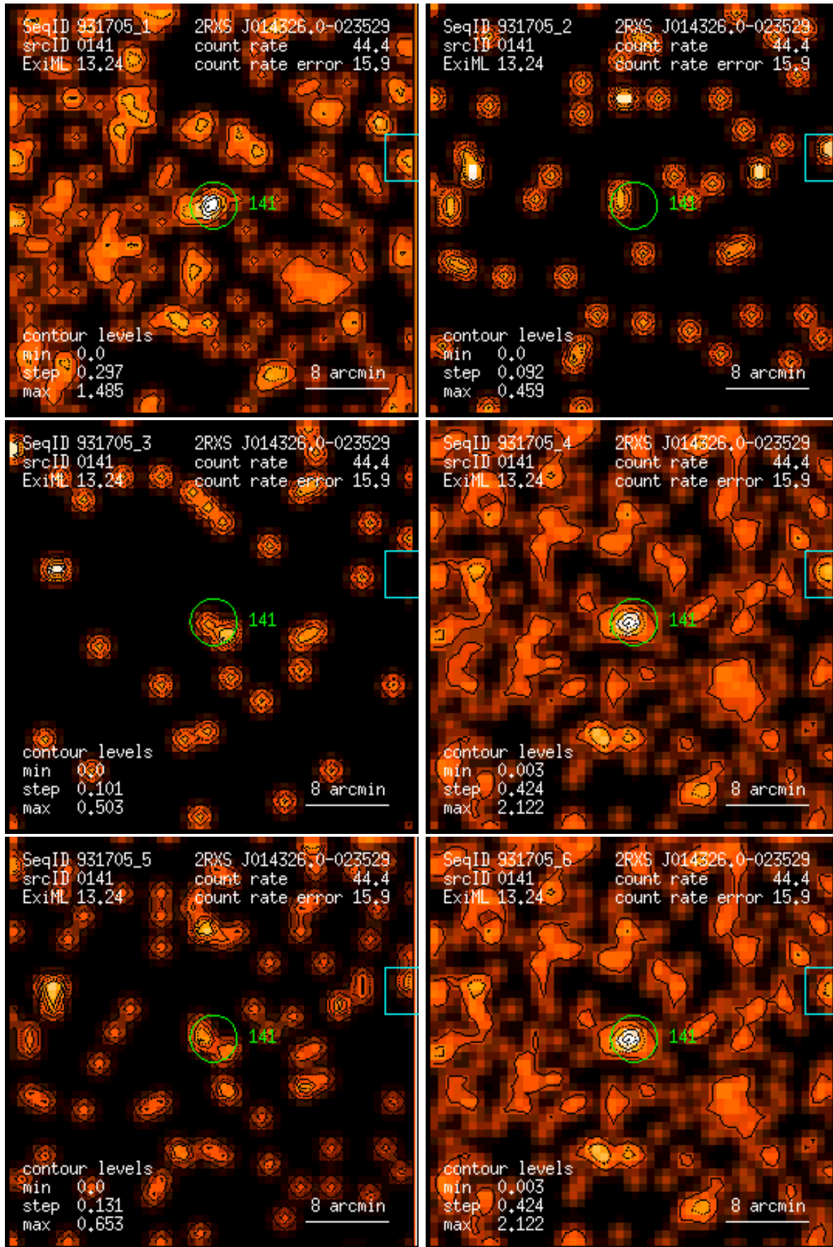
Figure 141: RASS 931705: detection 0141: band rate images, Gaussian filter: (1) PSPC channels 11 – 41, (2) 52 – 90, (3) 91 – 201, (4) 11 – 235, (5) 52 – 201, (6) 11 – 201. Broad band rates in counts/ks. Band rate contour levels in counts/ks/arcmin 2 .
