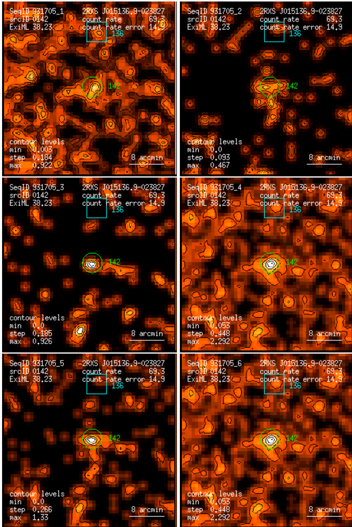
Figure 142: RASS 931705: detection 0142: band rate images, Gaussian filter: (1) PSPC channels 11 – 41, (2) 52 – 90, (3) 91 – 201, (4) 11 – 235, (5) 52 – 201, (6) 11 – 201. Broad band rates in counts/ks. Band rate contour levels in counts/ks/arcmin 2 .
