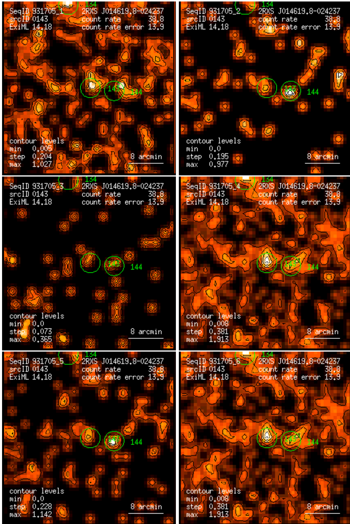
Figure 143: RASS 931705: detection 0143: band rate images, Gaussian filter: (1) PSPC channels 11 – 41, (2) 52 – 90, (3) 91 – 201, (4) 11 – 235, (5) 52 – 201, (6) 11 – 201. Broad band rates in counts/ks. Band rate contour levels in counts/ks/arcmin 2 .
