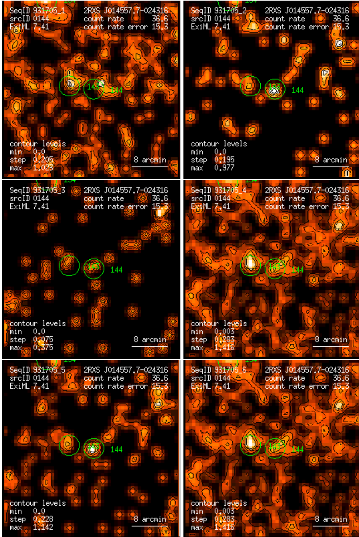
Figure 144: RASS 931705: detection 0144: band rate images, Gaussian filter: (1) PSPC channels 11 – 41, (2) 52 – 90, (3) 91 – 201, (4) 11 – 235, (5) 52 – 201, (6) 11 – 201. Broad band rates in counts/ks. Band rate contour levels in counts/ks/arcmin 2 .
