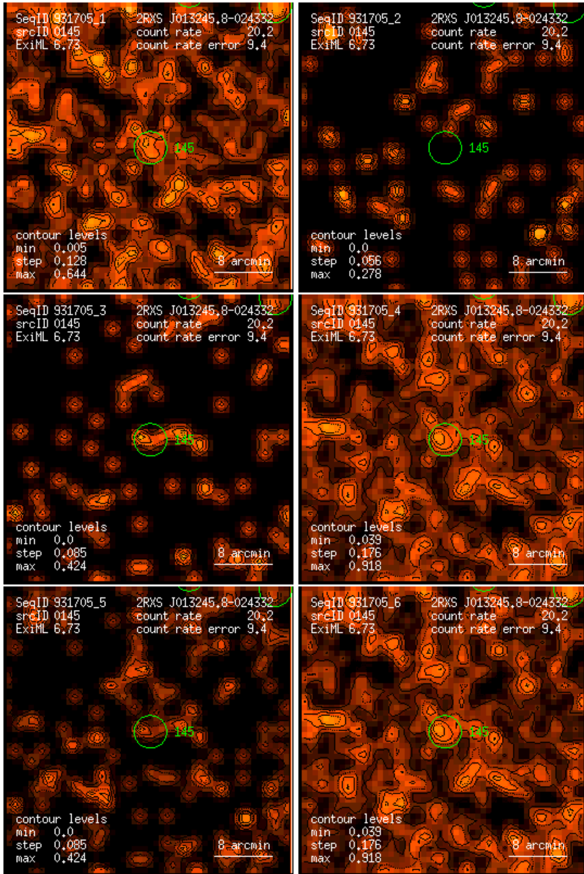
Figure 145: RASS 931705: detection 0145: band rate images, Gaussian filter: (1) PSPC channels 11 – 41, (2) 52 – 90, (3) 91 – 201, (4) 11 – 235, (5) 52 – 201, (6) 11 – 201. Broad band rates in counts/ks. Band rate contour levels in counts/ks/arcmin 2 .
