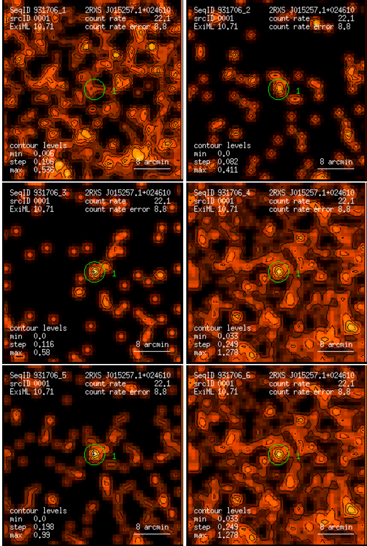
Figure 1: RASS 931706: detection 0001: band rate images, Gaussian filter: (1) PSPC channels 11 – 41, (2) 52 – 90, (3) 91 – 201, (4) 11 – 235, (5) 52 – 201, (6) 11 – 201. Broad band rates in counts/ks. Band rate contour levels in counts/ks/arcmin 2 .
