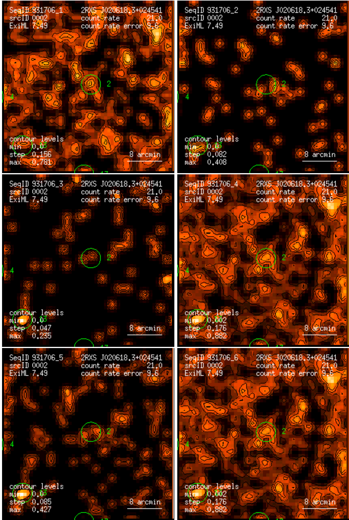
Figure 2: RASS 931706: detection 0002: band rate images, Gaussian filter: (1) PSPC channels 11 – 41, (2) 52 – 90, (3) 91 – 201, (4) 11 – 235, (5) 52 – 201, (6) 11 – 201. Broad band rates in counts/ks. Band rate contour levels in counts/ks/arcmin 2 .
