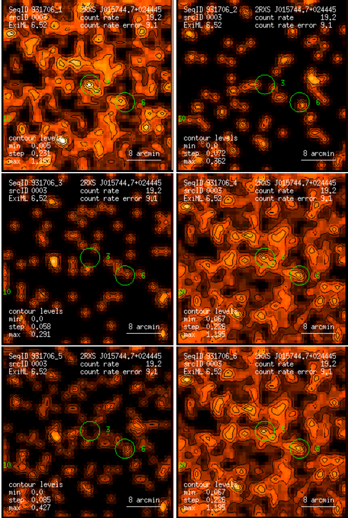
Figure 3: RASS 931706: detection 0003: band rate images, Gaussian filter: (1) PSPC channels 11 – 41, (2) 52 – 90, (3) 91 – 201, (4) 11 – 235, (5) 52 – 201, (6) 11 – 201. Broad band rates in counts/ks. Band rate contour levels in counts/ks/arcmin 2 .
