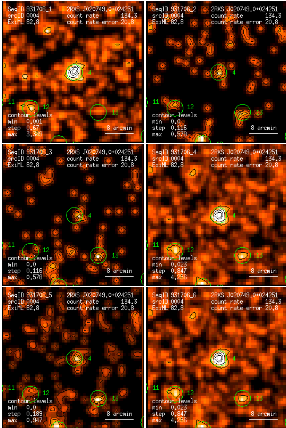
Figure 4: RASS 931706: detection 0004: band rate images, Gaussian filter: (1) PSPC channels 11 – 41, (2) 52 – 90, (3) 91 – 201, (4) 11 – 235, (5) 52 – 201, (6) 11 – 201. Broad band rates in counts/ks. Band rate contour levels in counts/ks/arcmin 2 .
