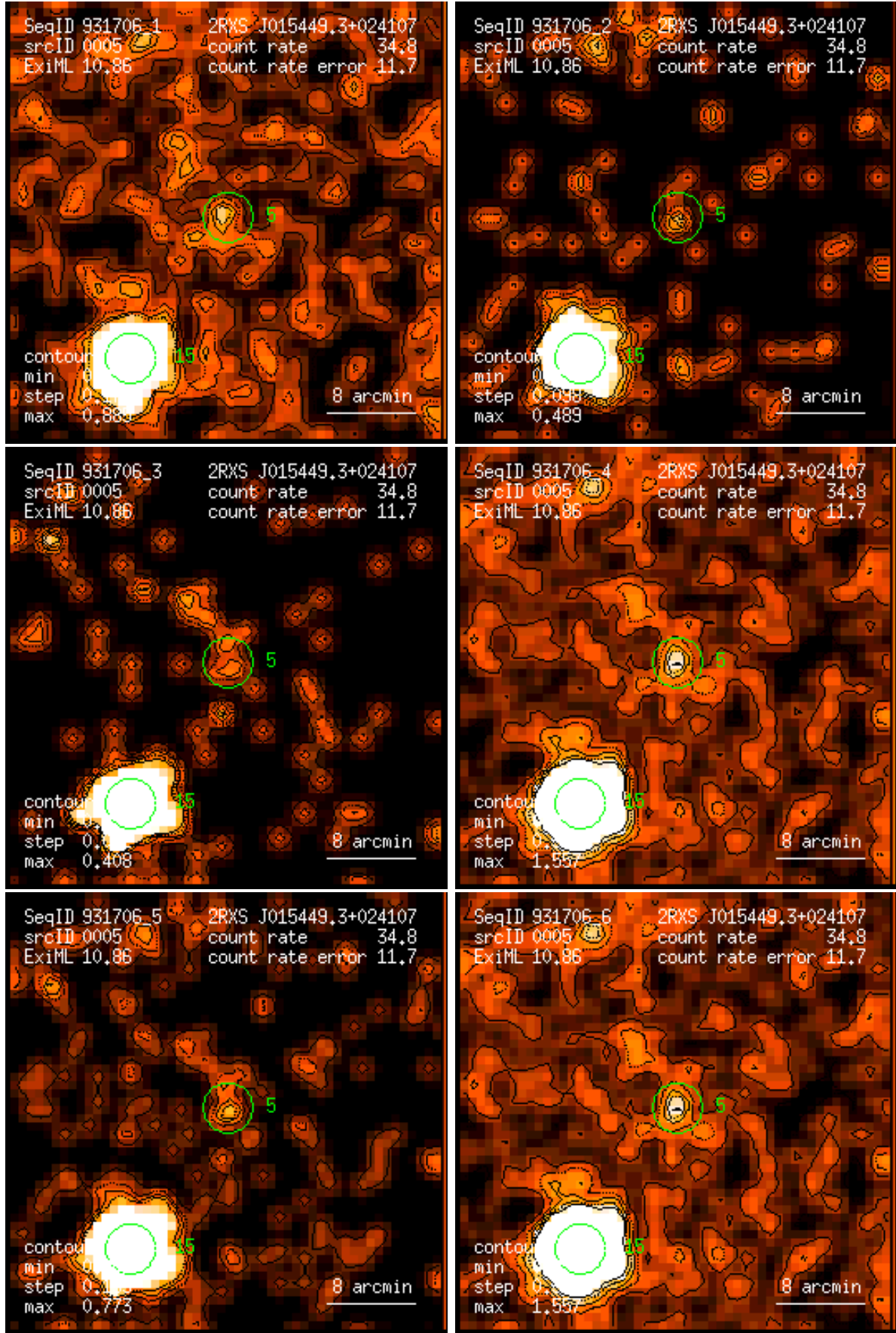
Figure 5: RASS 931706: detection 0005: band rate images, Gaussian filter: (1) PSPC channels 11 – 41, (2) 52 – 90, (3) 91 – 201, (4) 11 – 235, (5) 52 – 201, (6) 11 – 201. Broad band rates in counts/ks. Band rate contour levels in counts/ks/arcmin 2 .
