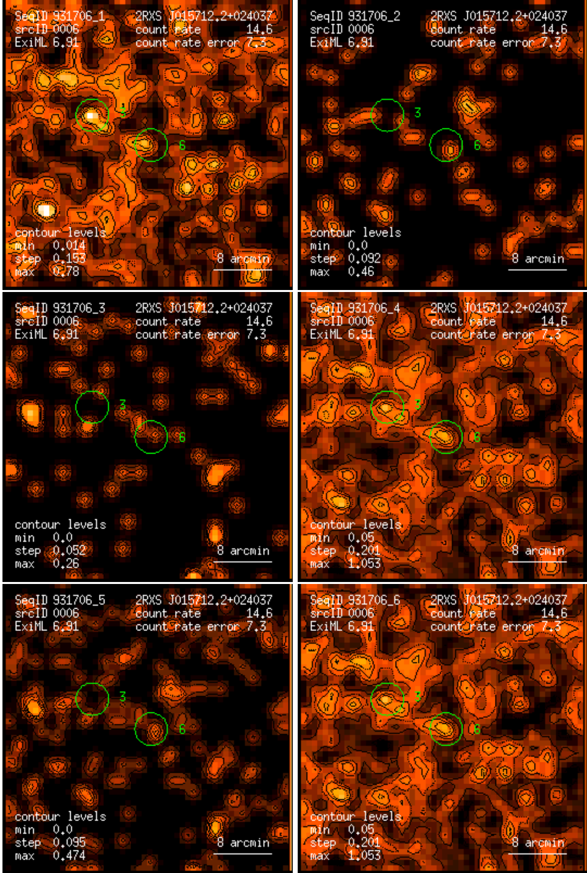
Figure 6: RASS 931706: detection 0006: band rate images, Gaussian filter: (1) PSPC channels 11 – 41, (2) 52 – 90, (3) 91 – 201, (4) 11 – 235, (5) 52 – 201, (6) 11 – 201. Broad band rates in counts/ks. Band rate contour levels in counts/ks/arcmin 2 .
