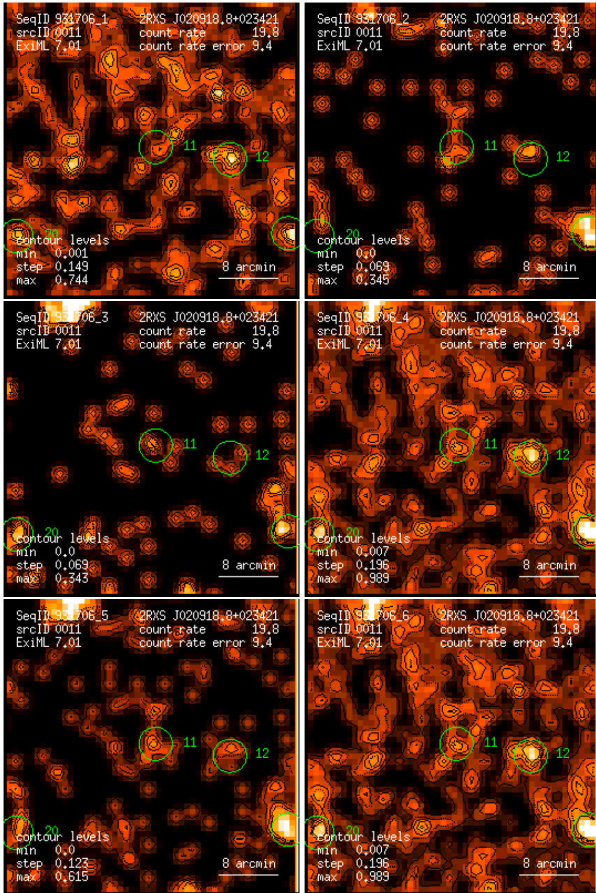
Figure 11: RASS 931706: detection 0011: band rate images, Gaussian filter: (1) PSPC channels 11 – 41, (2) 52 – 90, (3) 91 – 201, (4) 11 – 235, (5) 52 – 201, (6) 11 – 201. Broad band rates in counts/ks. Band rate contour levels in counts/ks/arcmin 2 .
