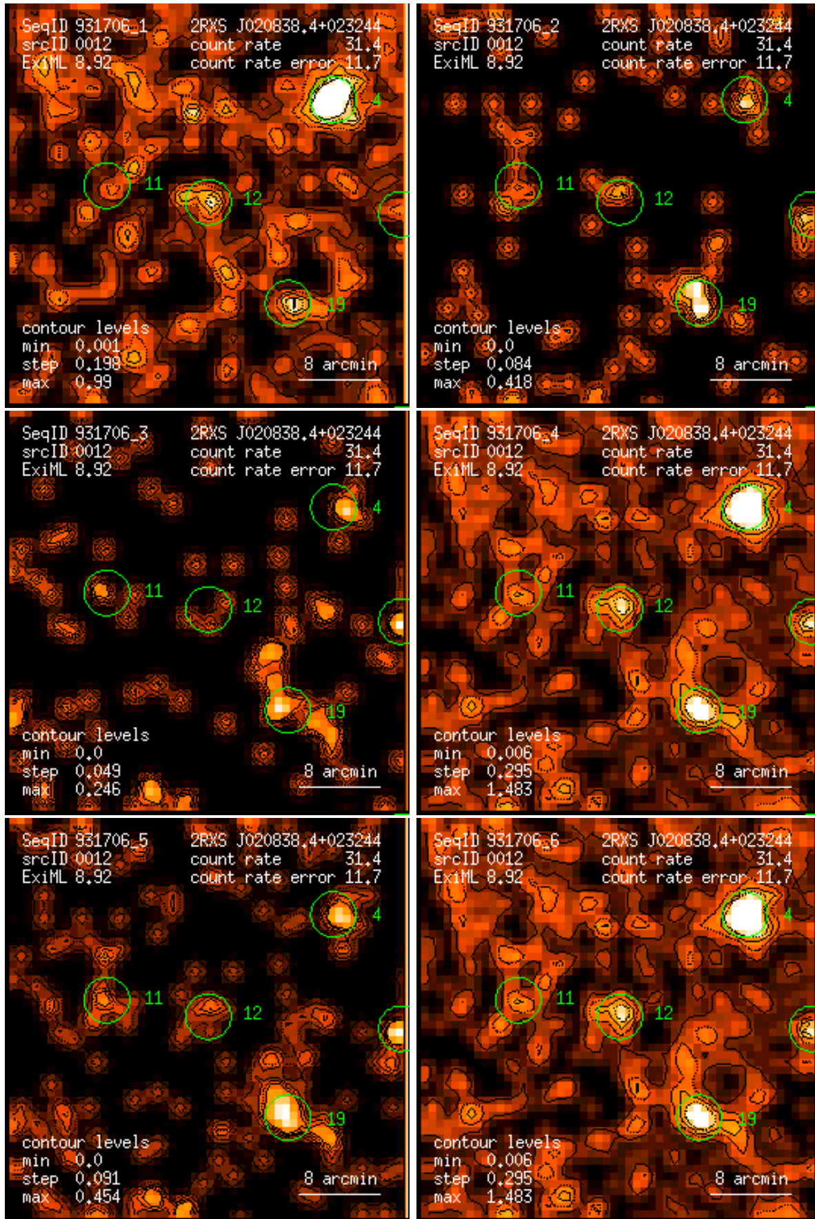
Figure 12: RASS 931706: detection 0012: band rate images, Gaussian filter: (1) PSPC channels 11 – 41, (2) 52 – 90, (3) 91 – 201, (4) 11 – 235, (5) 52 – 201, (6) 11 – 201. Broad band rates in counts/ks. Band rate contour levels in counts/ks/arcmin 2 .
