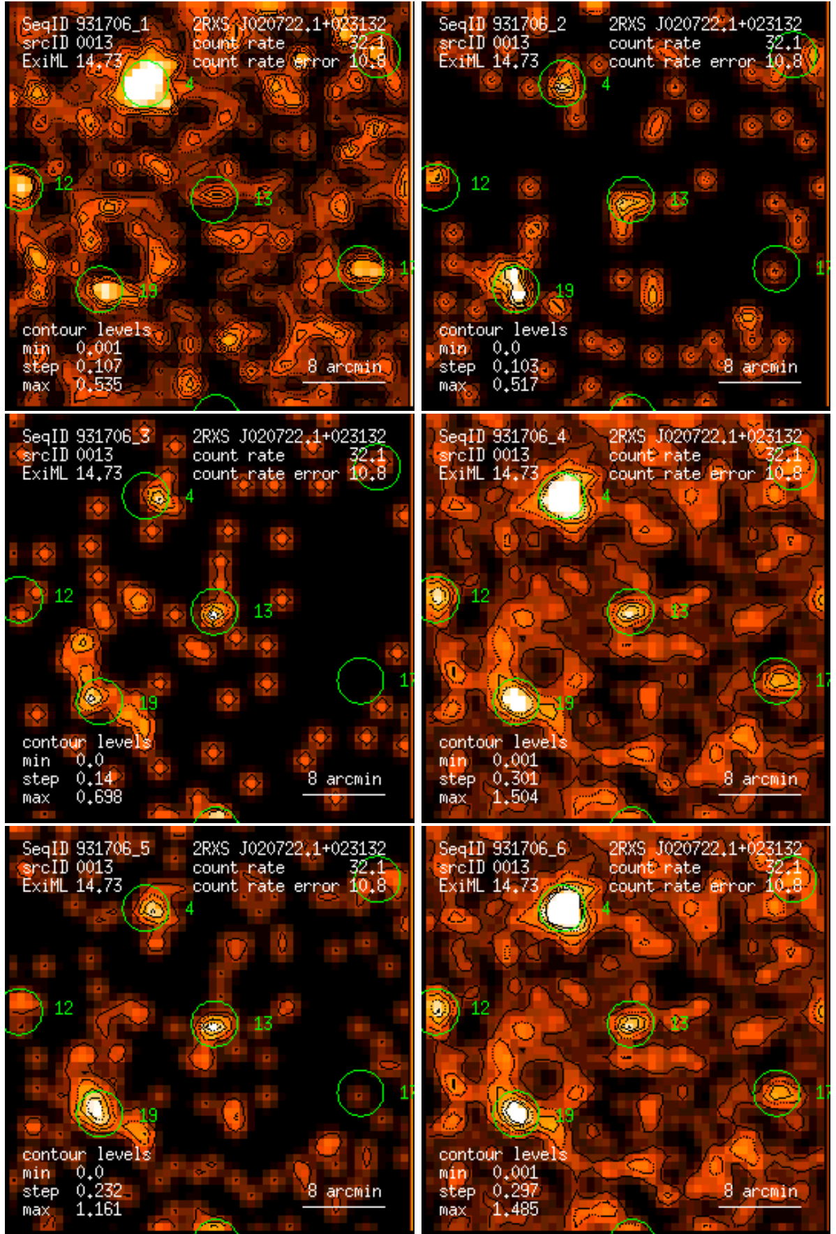
Figure 13: RASS 931706: detection 0013: band rate images, Gaussian filter: (1) PSPC channels 11 – 41, (2) 52 – 90, (3) 91 – 201, (4) 11 – 235, (5) 52 – 201, (6) 11 – 201. Broad band rates in counts/ks. Band rate contour levels in counts/ks/arcmin 2 .
