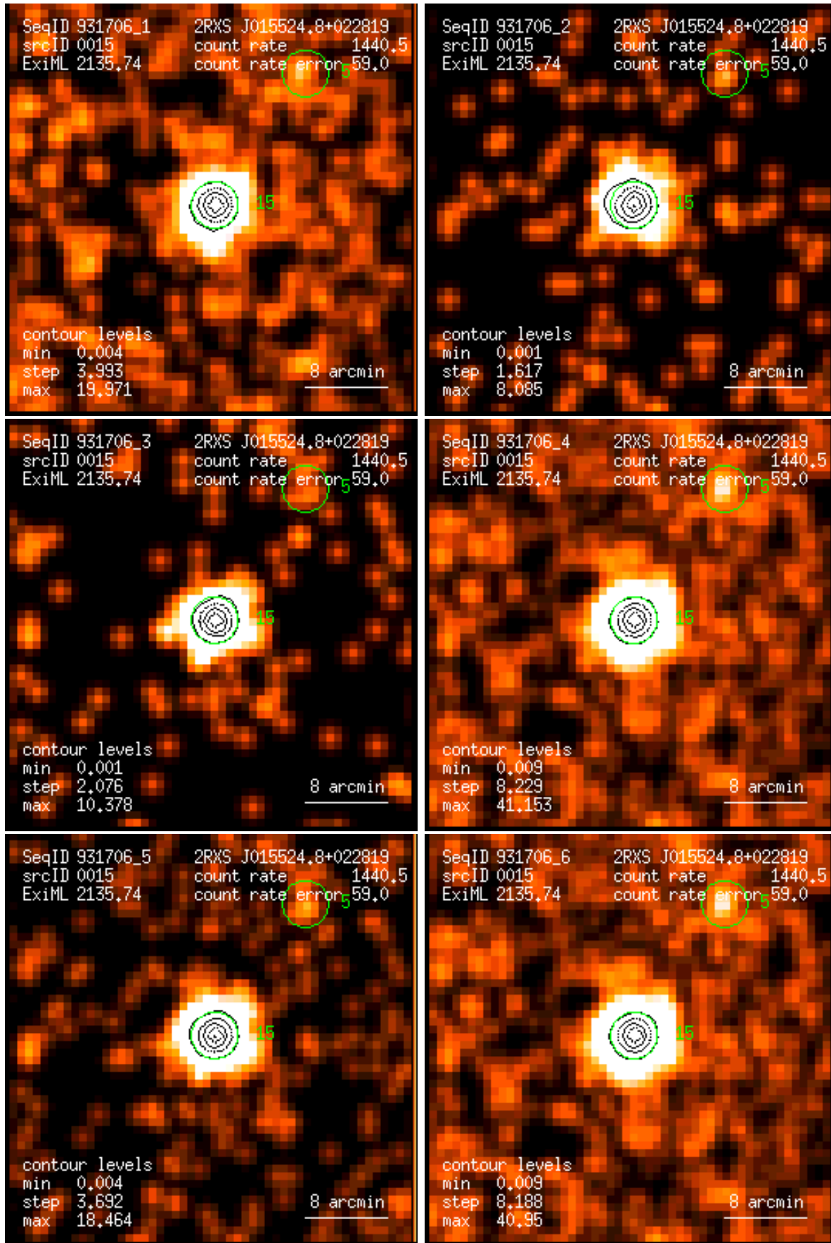
Figure 15: RASS 931706: detection 0015: band rate images, Gaussian filter: (1) PSPC channels 11 – 41, (2) 52 – 90, (3) 91 – 201, (4) 11 – 235, (5) 52 – 201, (6) 11 – 201. Broad band rates in counts/ks. Band rate contour levels in counts/ks/arcmin 2 .
