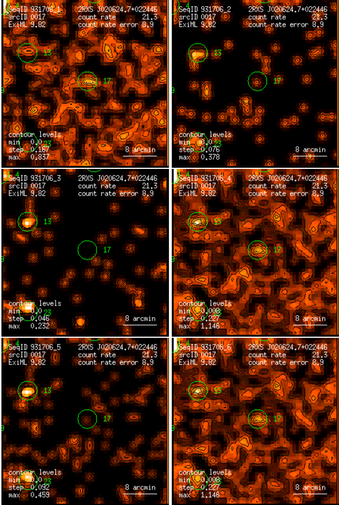
Figure 17: RASS 931706: detection 0017: band rate images, Gaussian filter: (1) PSPC channels 11 – 41, (2) 52 – 90, (3) 91 – 201, (4) 11 – 235, (5) 52 – 201, (6) 11 – 201. Broad band rates in counts/ks. Band rate contour levels in counts/ks/arcmin 2 .
