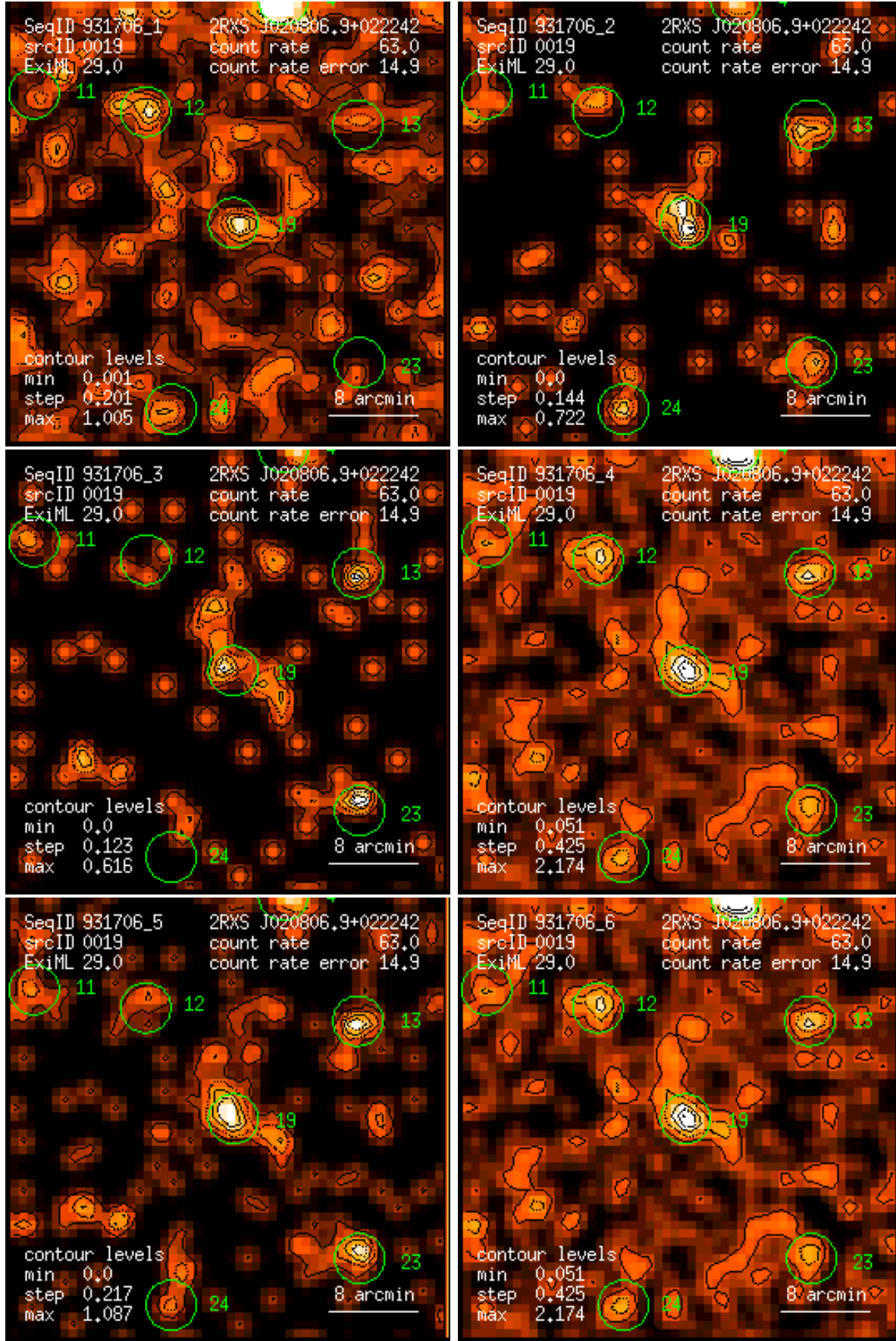
Figure 19: RASS 931706: detection 0019: band rate images, Gaussian filter: (1) PSPC channels 11 – 41, (2) 52 – 90, (3) 91 – 201, (4) 11 – 235, (5) 52 – 201, (6) 11 – 201. Broad band rates in counts/ks. Band rate contour levels in counts/ks/arcmin 2 .
