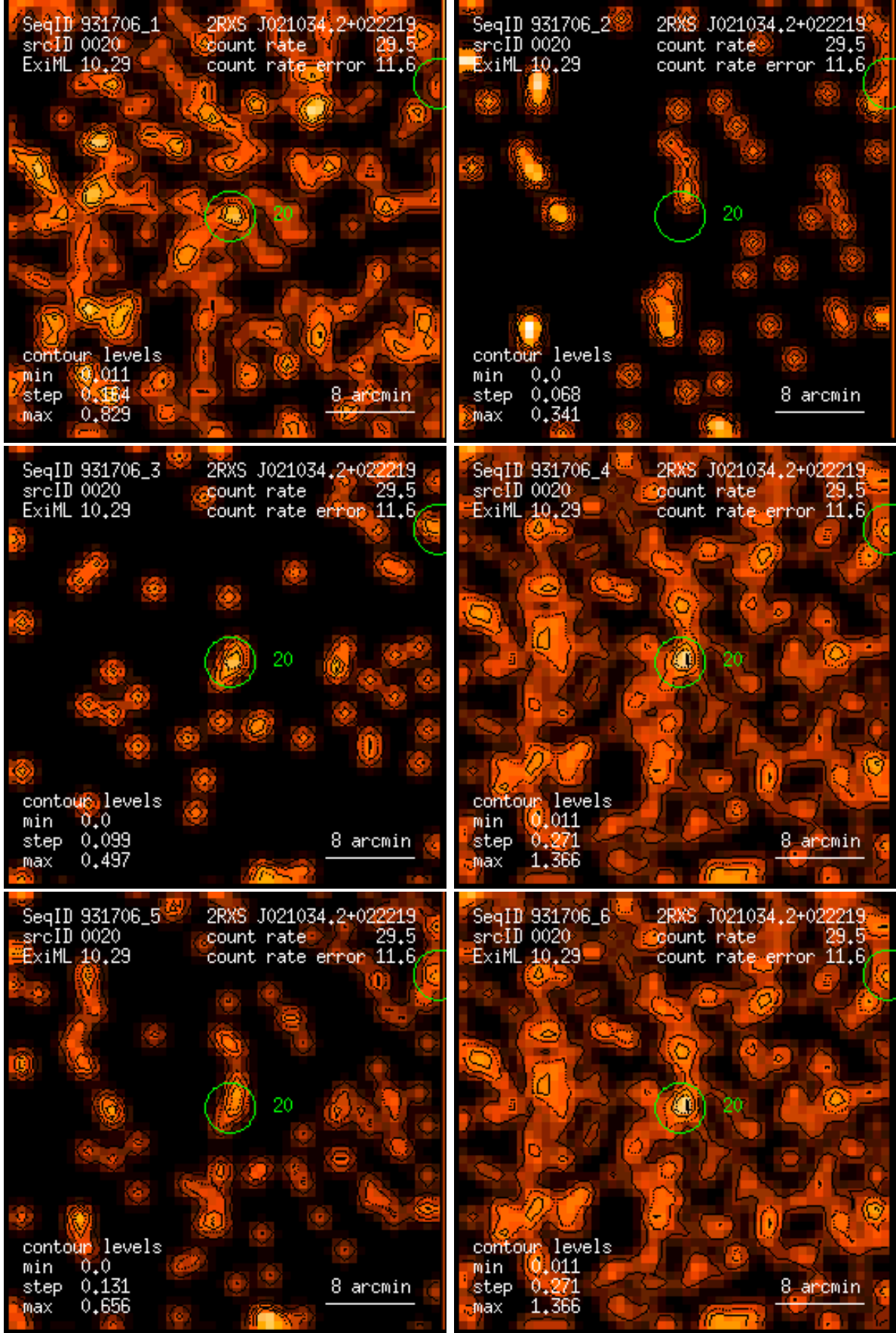
Figure 20: RASS 931706: detection 0020: band rate images, Gaussian filter: (1) PSPC channels 11 – 41, (2) 52 – 90, (3) 91 – 201, (4) 11 – 235, (5) 52 – 201, (6) 11 – 201. Broad band rates in counts/ks. Band rate contour levels in counts/ks/arcmin 2 .
