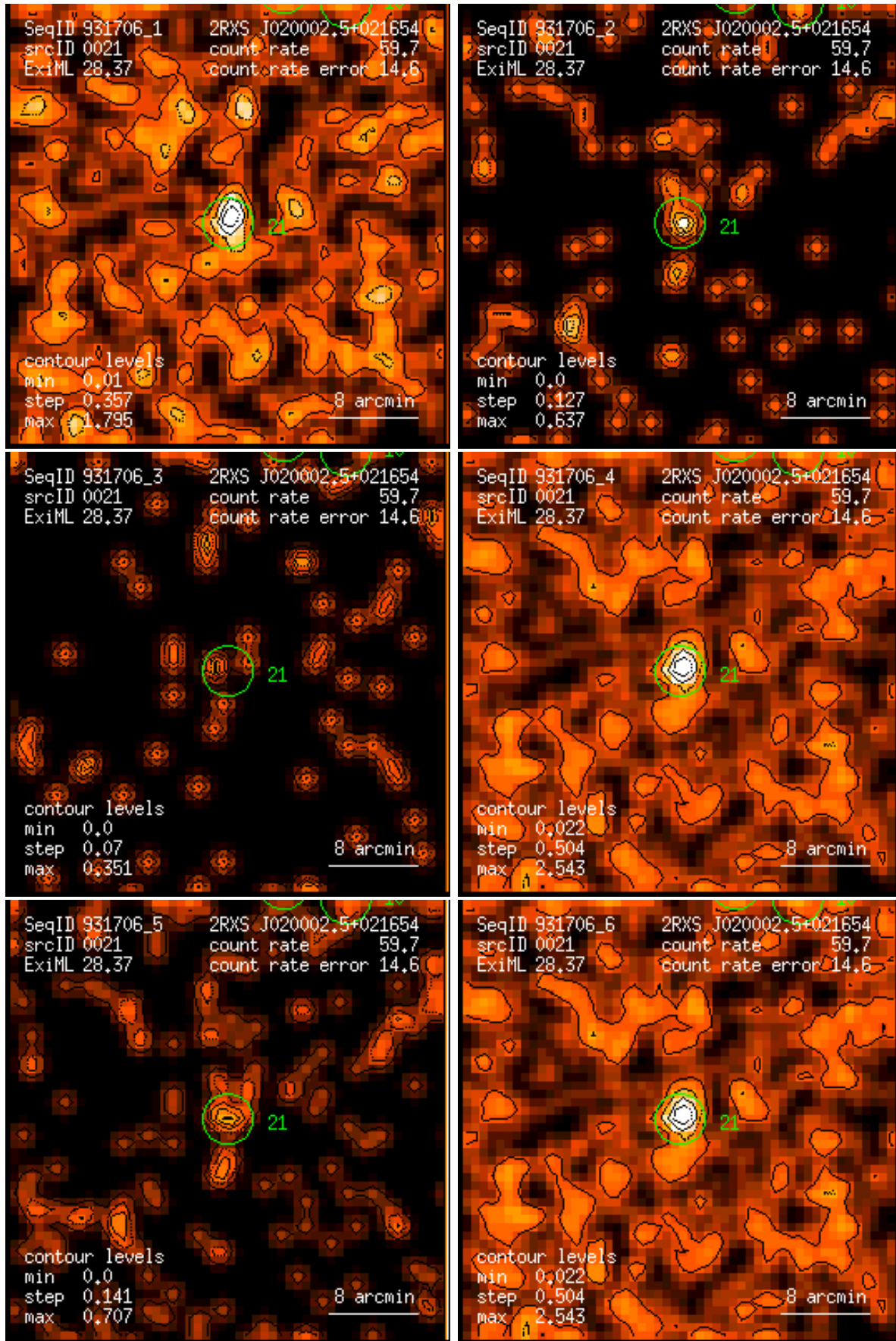
Figure 21: RASS 931706: detection 0021: band rate images, Gaussian filter: (1) PSPC channels 11 – 41, (2) 52 – 90, (3) 91 – 201, (4) 11 – 235, (5) 52 – 201, (6) 11 – 201. Broad band rates in counts/ks. Band rate contour levels in counts/ks/arcmin 2 .
